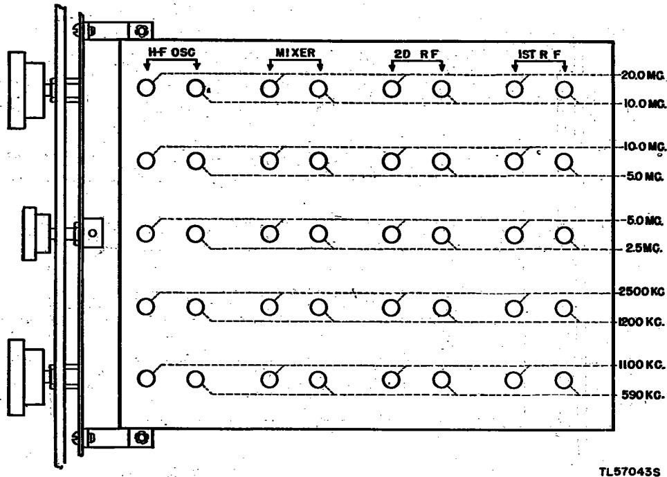
Figure 48. Radio Receiver BC-1004-(*), alinement chart.
