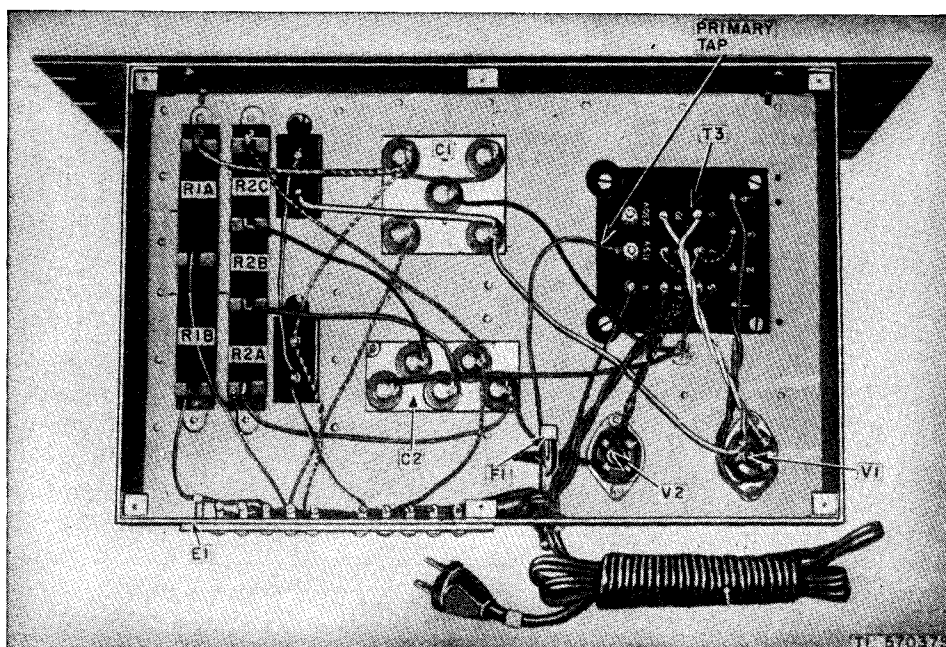
Figure 44. Power Supply Unit RA-94-A, chassis, bottom view.
