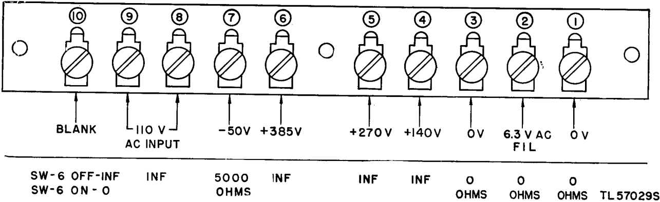
Figure 36. Receiver terminal strip, voltage and resistance measurements.
