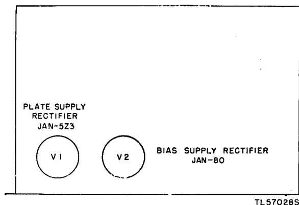
Figure 14. Power supply unit, tube location.
