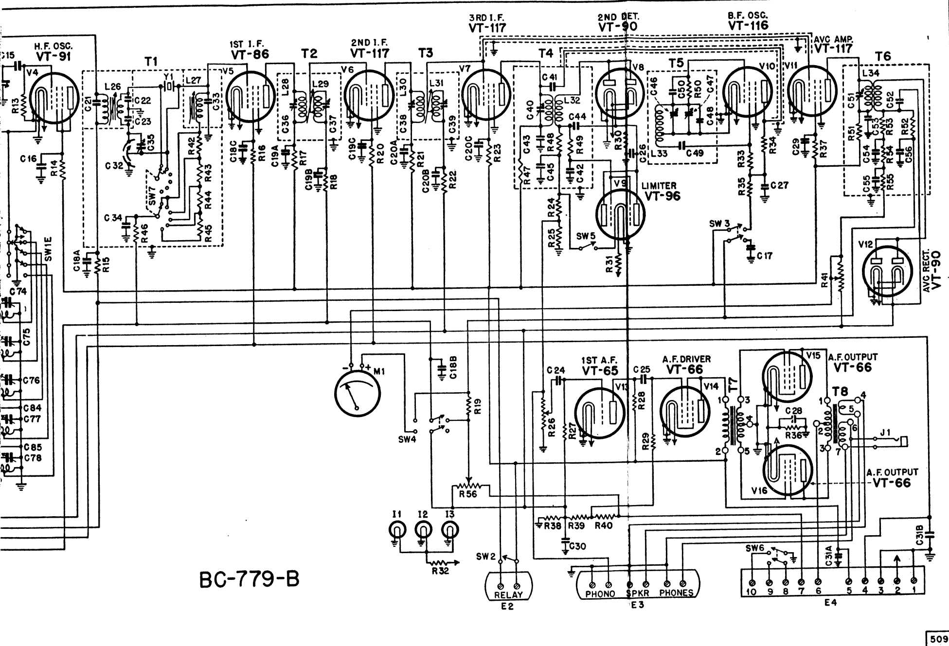
Figure 24. Radio Receiver BC-779-B Circuit Diagram
