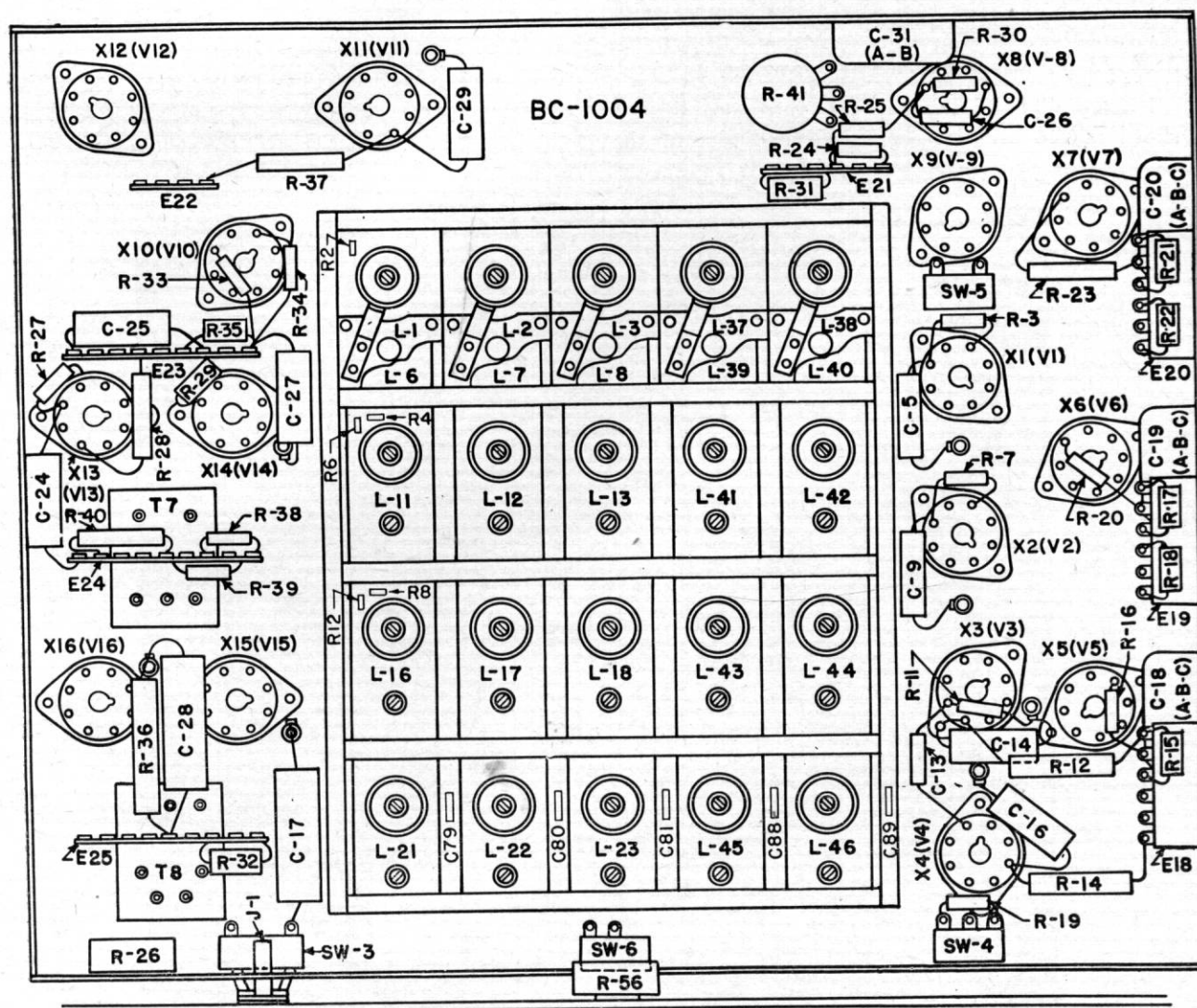
Figure 40. Radio Receiver BC-1004-(*), chassis, bottom view.
