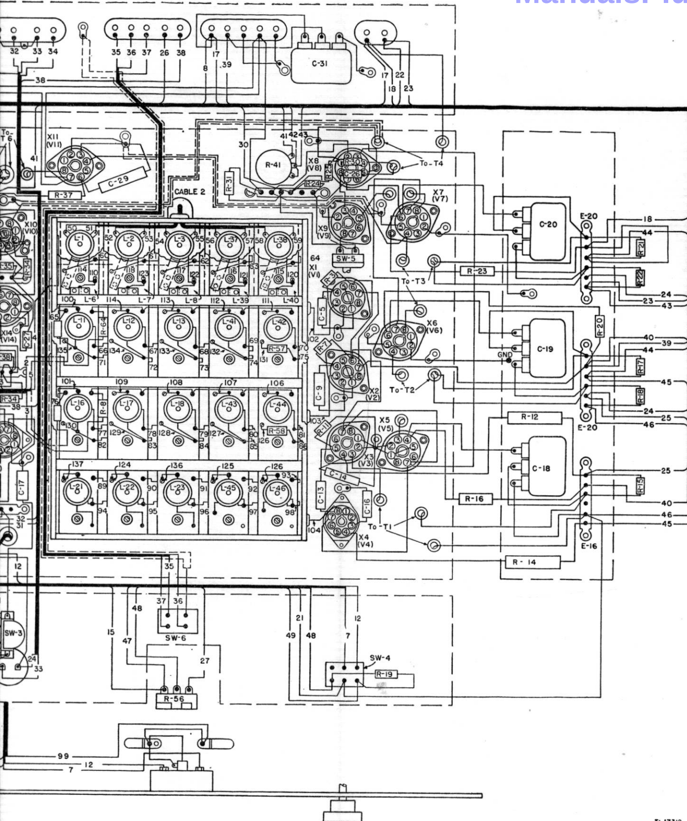
Figure 60. Receiver chassis, wiring diagram.
