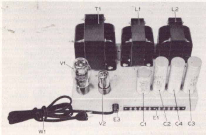
FIG. 6—Top view of power supply.
