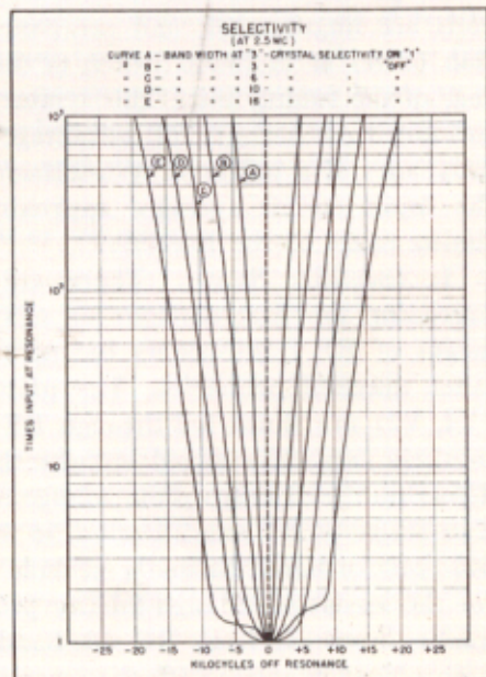
FIG. 8—Selectivity curves.
