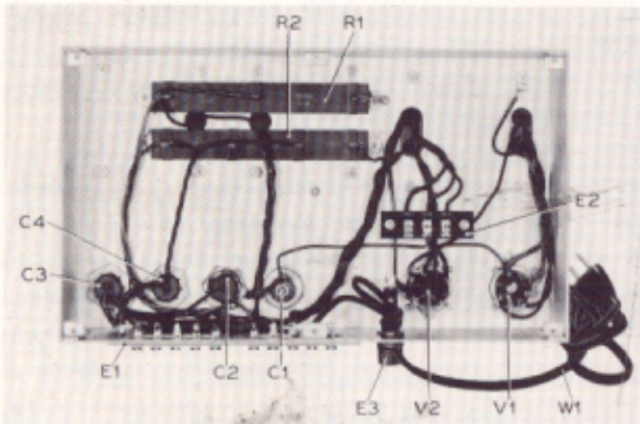
FIG. 5—Bottom view of power supply.
