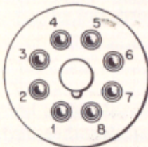
OCTAL BASE
