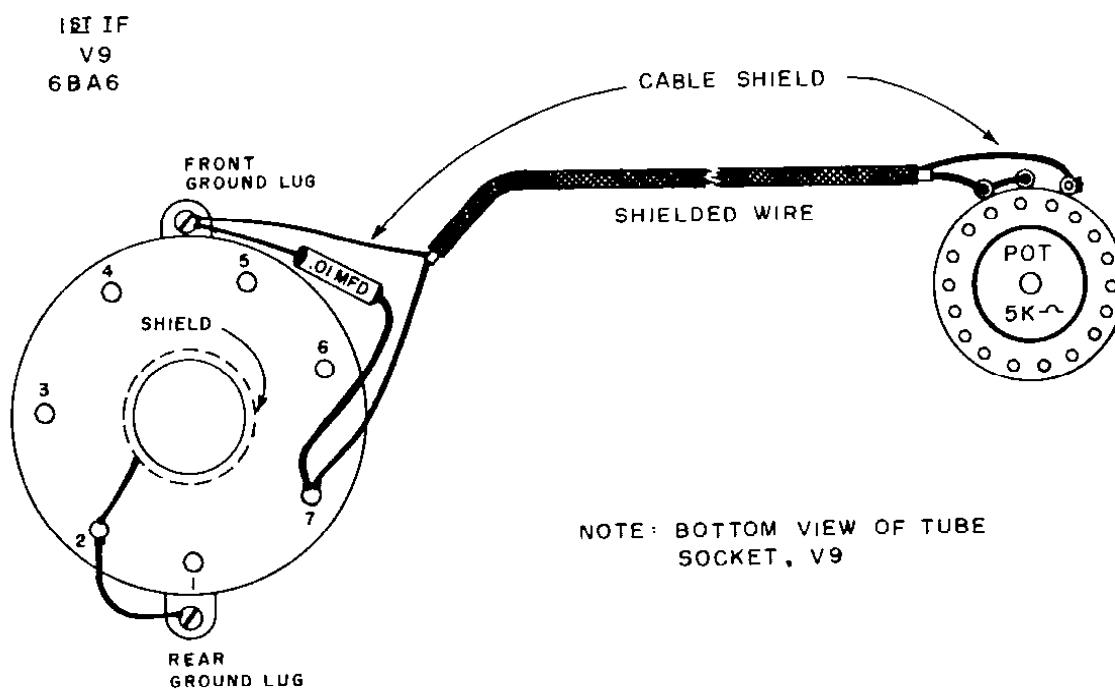
Figure 2. Installation of IF Gain Control
