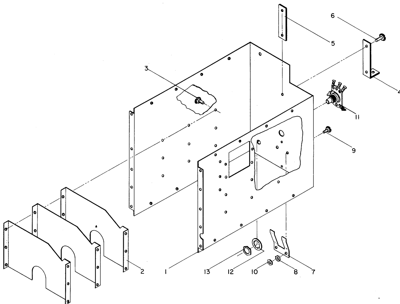
Figure 10. Tuning Unit Shield Assembly
