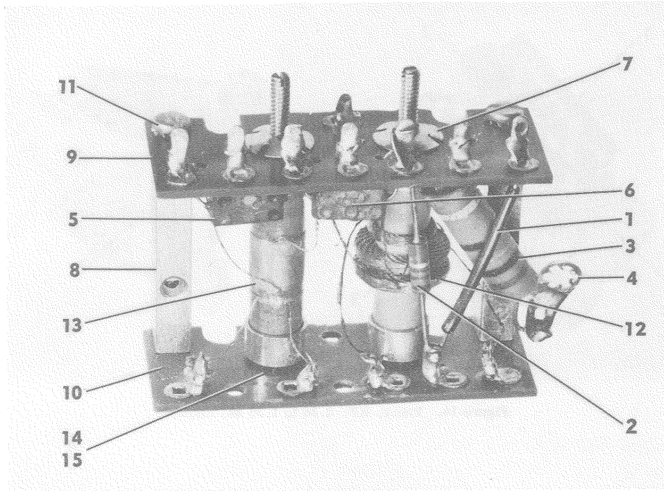
Figure 13. Mixer Plate Coil Assembly
