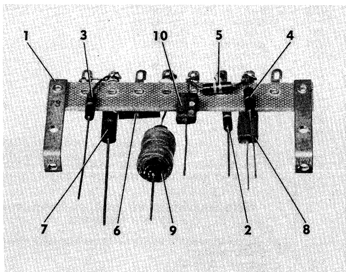
Figure 35. Resistor-Capacitor Subassembly
