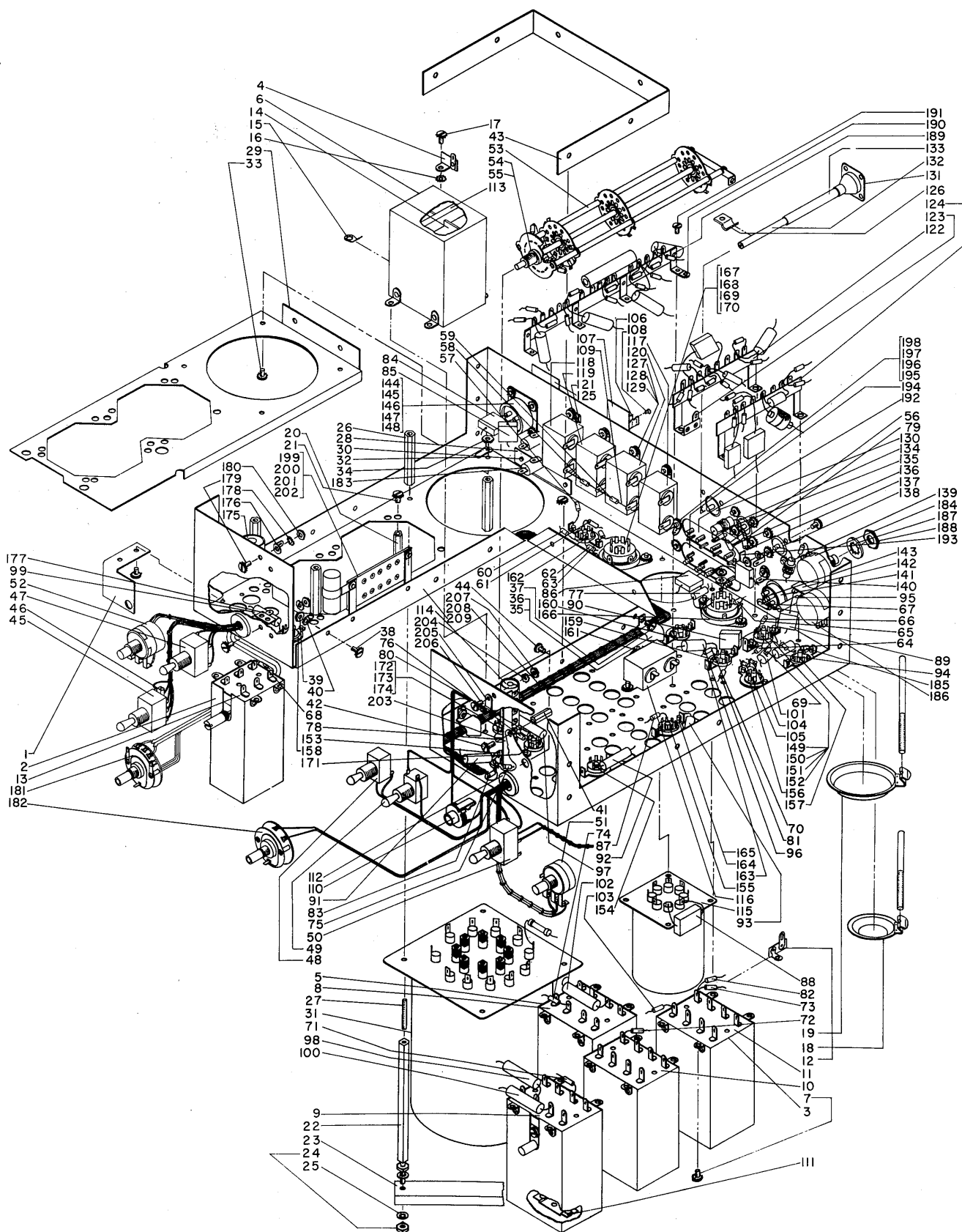
Figure 32. Chassis Assembly
