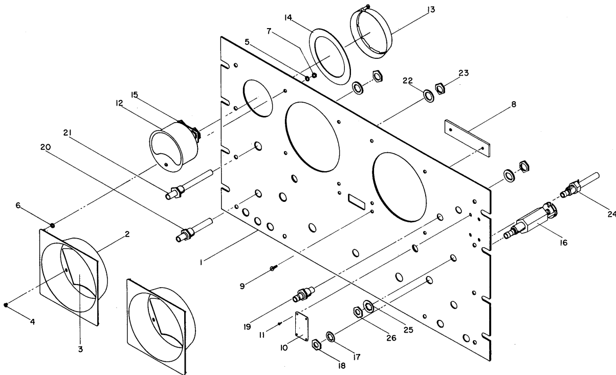
Figure 6. Panel Assembly
