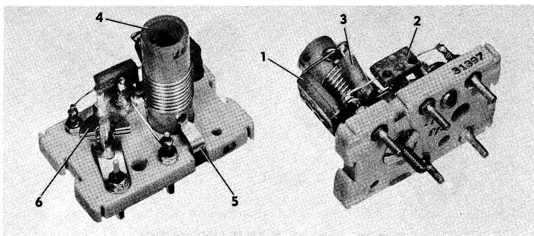
Figure 28. Tuner, RF: 14.8 to 29.7 MC (H-F Osc)
