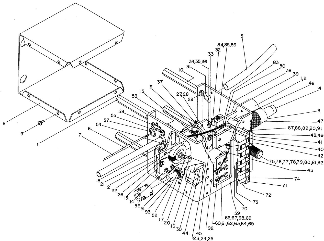
Figure 4. Frequency Control Unit Assembly
