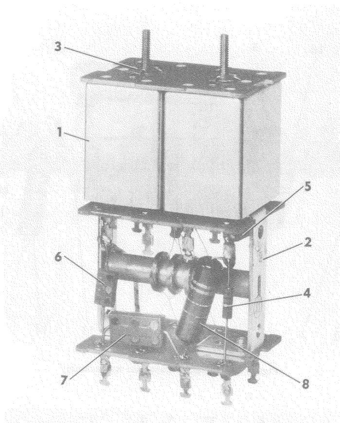
Figure 38. Transformer, IF
