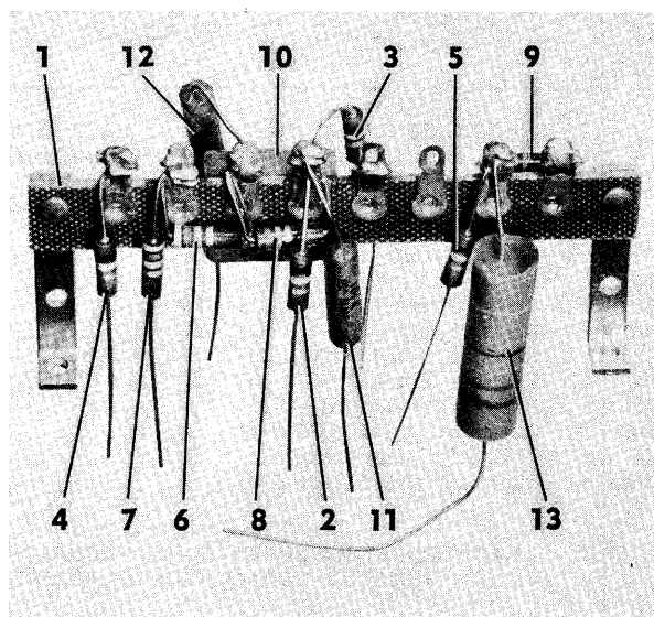
Figure 34. Resistor-Capacitor Subassembly
