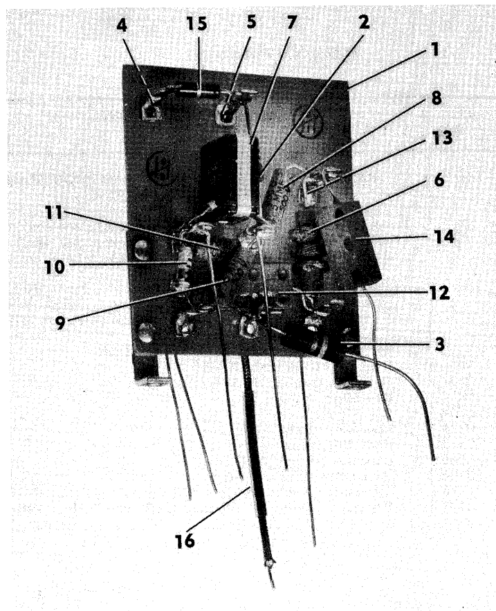
Figure 37. 3.5-MC Oscillator
