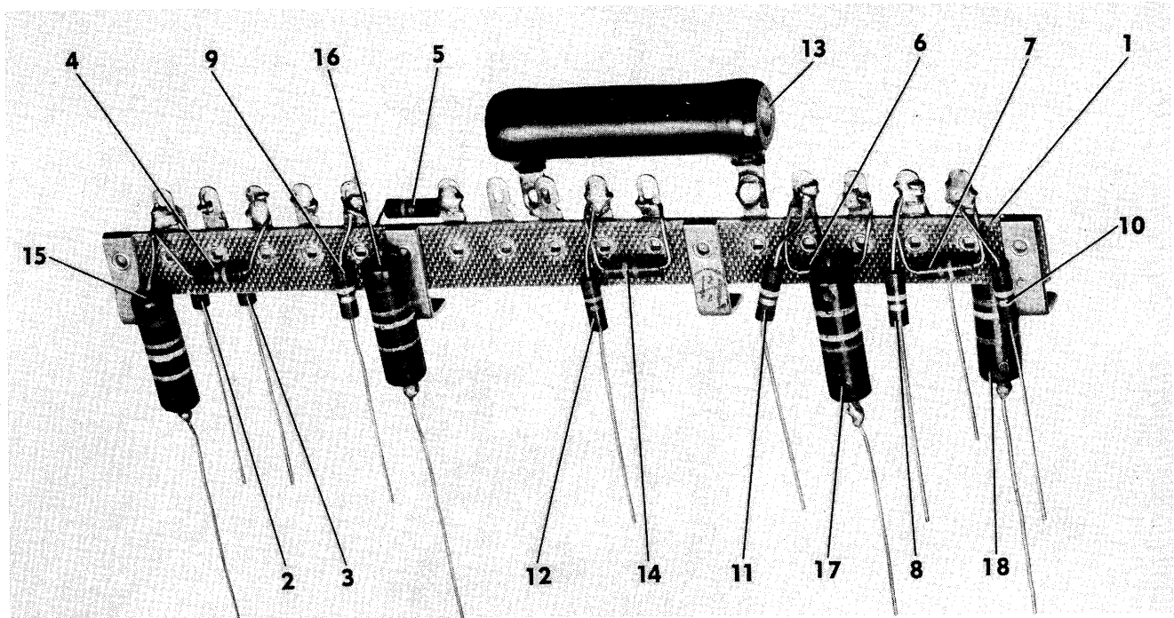
Figure 36. Resistor-Capacitor Subassembly
