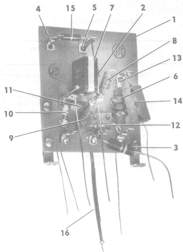
Figure 37. 3.5-MC Oscillator
