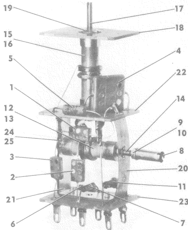
Figure 41. Beat-frequency Oscillator
