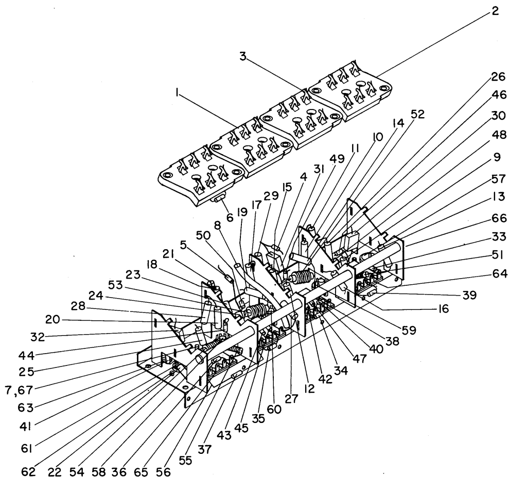
Figure 12. R-F Wiring Assembly
