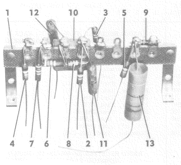
Figure 34. Resistor-Capacitor Subassembly
