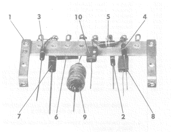
Figure 35. Resistor-Capacitor Subassembly
