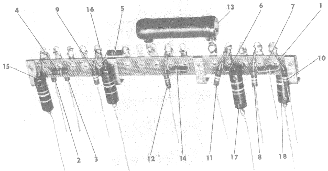
Figure 36. Resistor-Capacitor Subassembly
