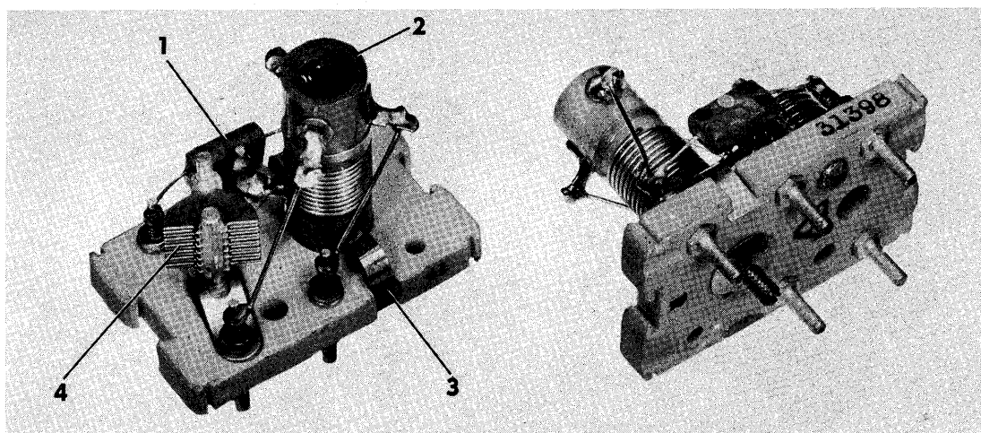
Figure 27. Tuner, RF: 14.8 to 29.7 MC (Interstage)
