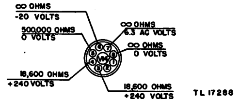
Figure 46. Radio Receivers BC-779-B, BC-794-B, and BC-1004-C, schematic diagram of a-f driver stage.
