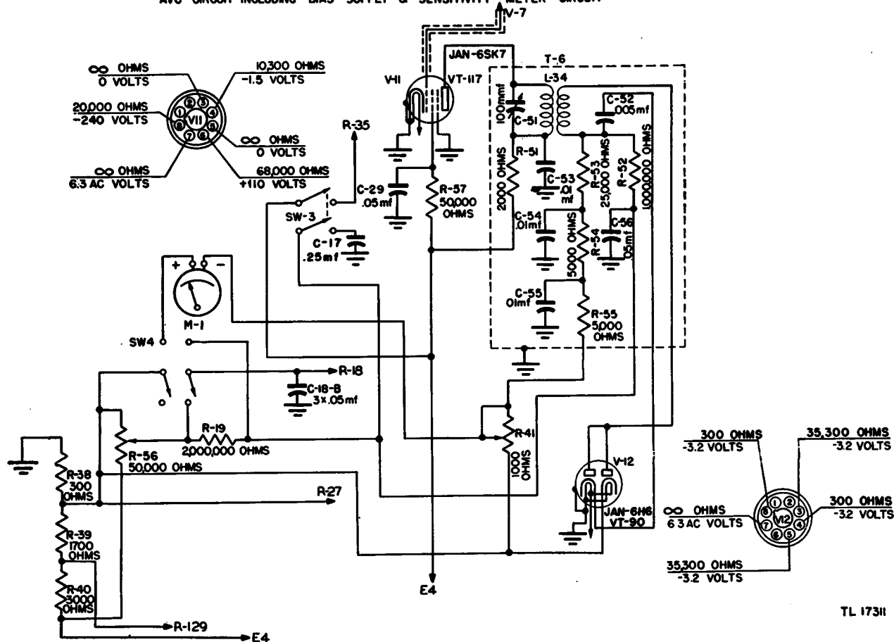
Figure 43. Radio Receivers BC-779-B, BC-794-B, and BC-1004-C, schematic diagram of a-v-c, bias supply, and sensitivity meter circuit.
