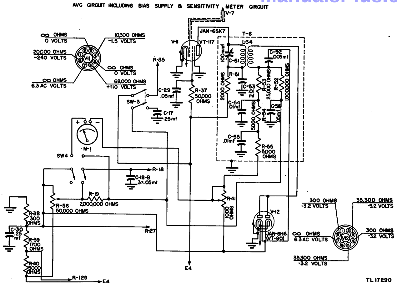
Figure 44. Radio Receiver BC-779-B, schematic diagram of a-v-c, bias supply, and sensitivity meter circuit.
