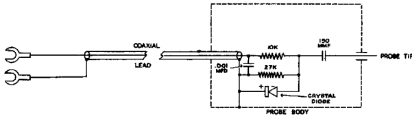
DEMOMULATOR PROBE 337-C
