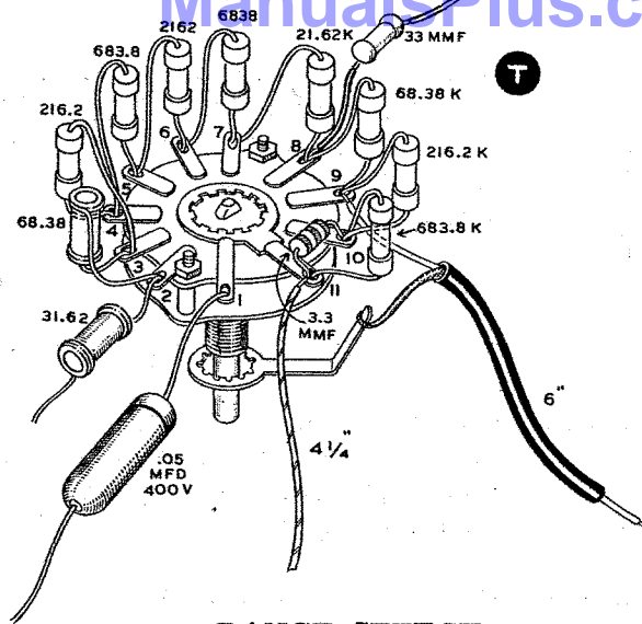
RANGE SWITCH
