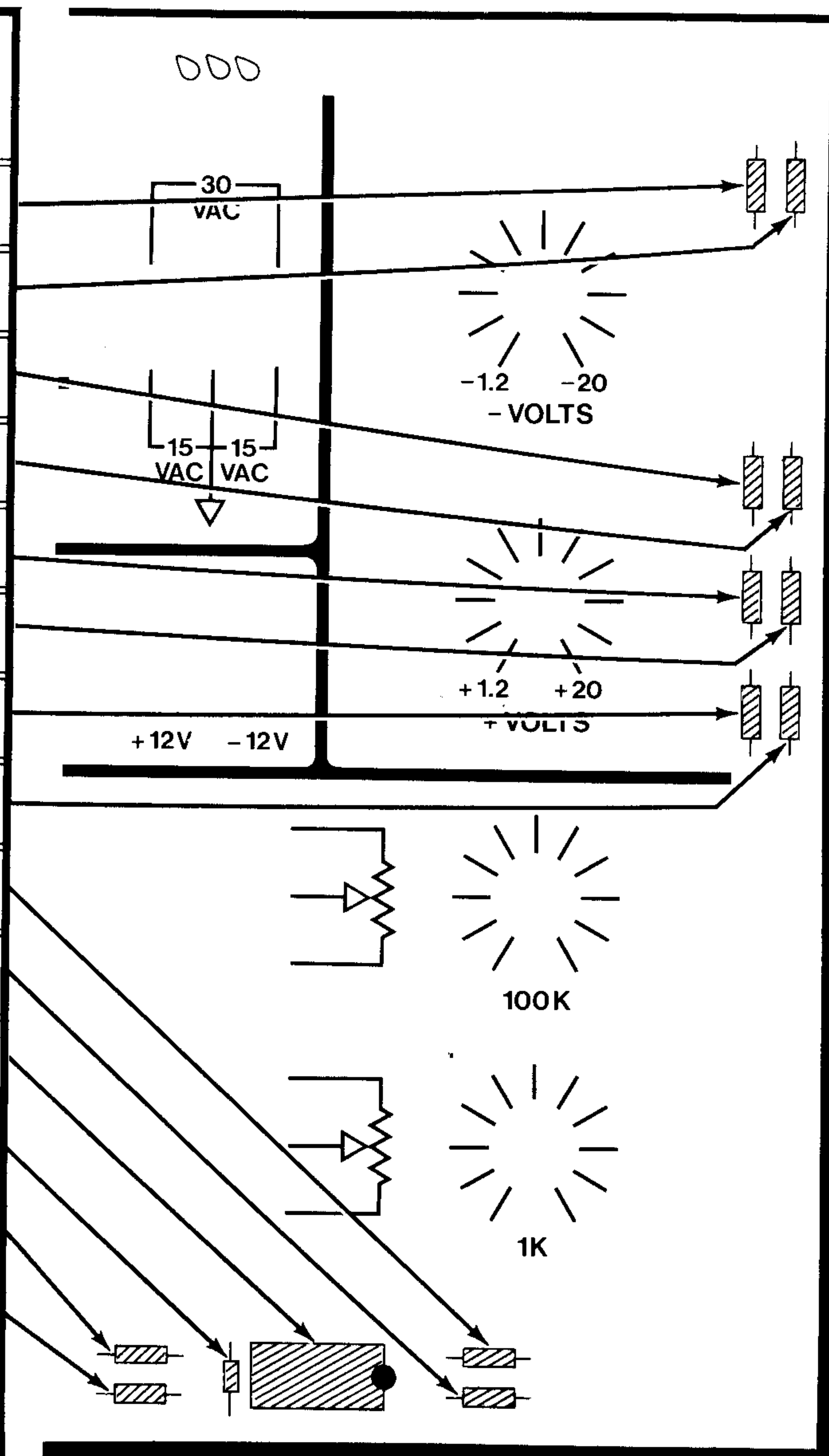
PICTORIAL 2-5
