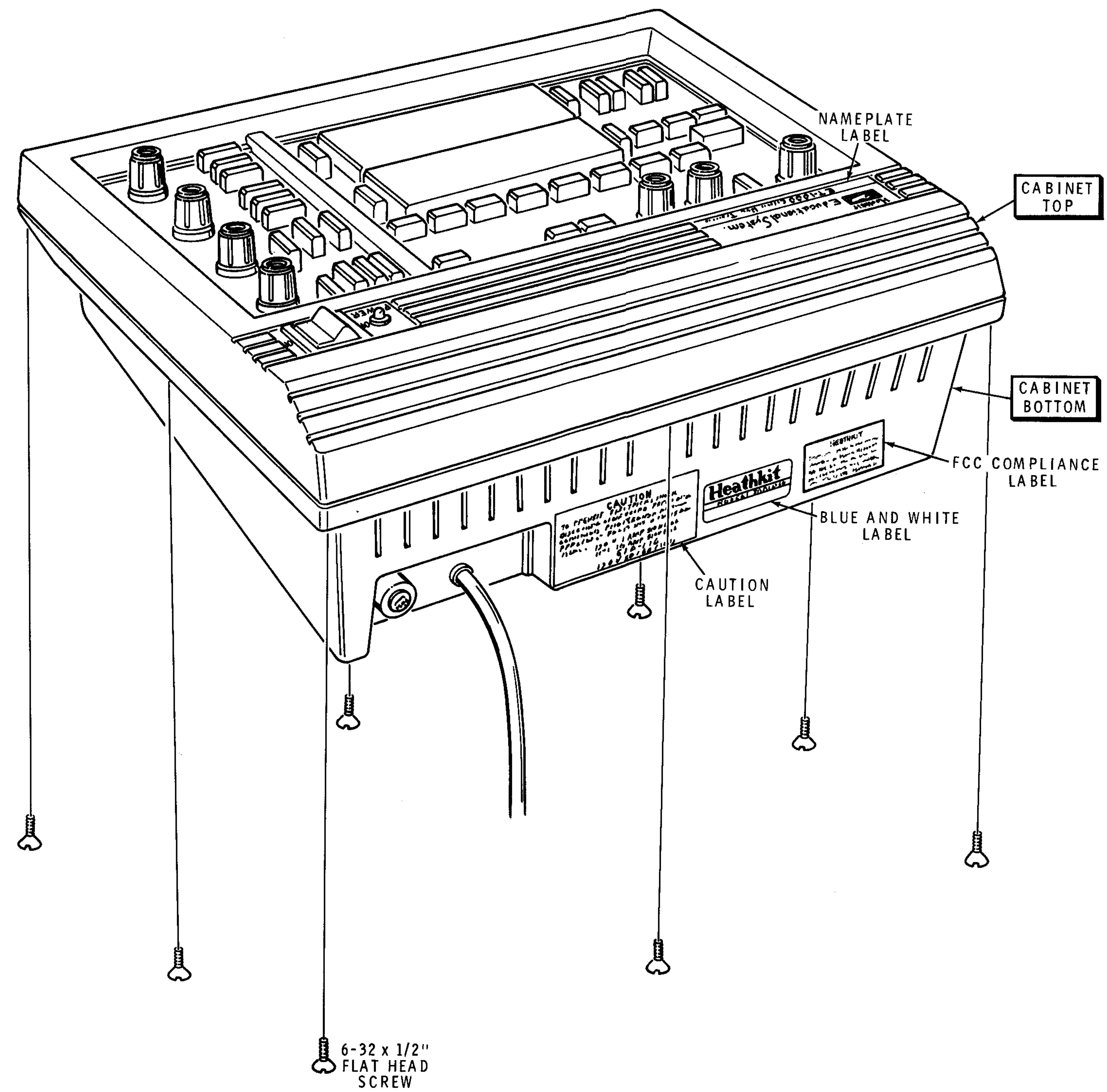
PICTORIAL 4-1
