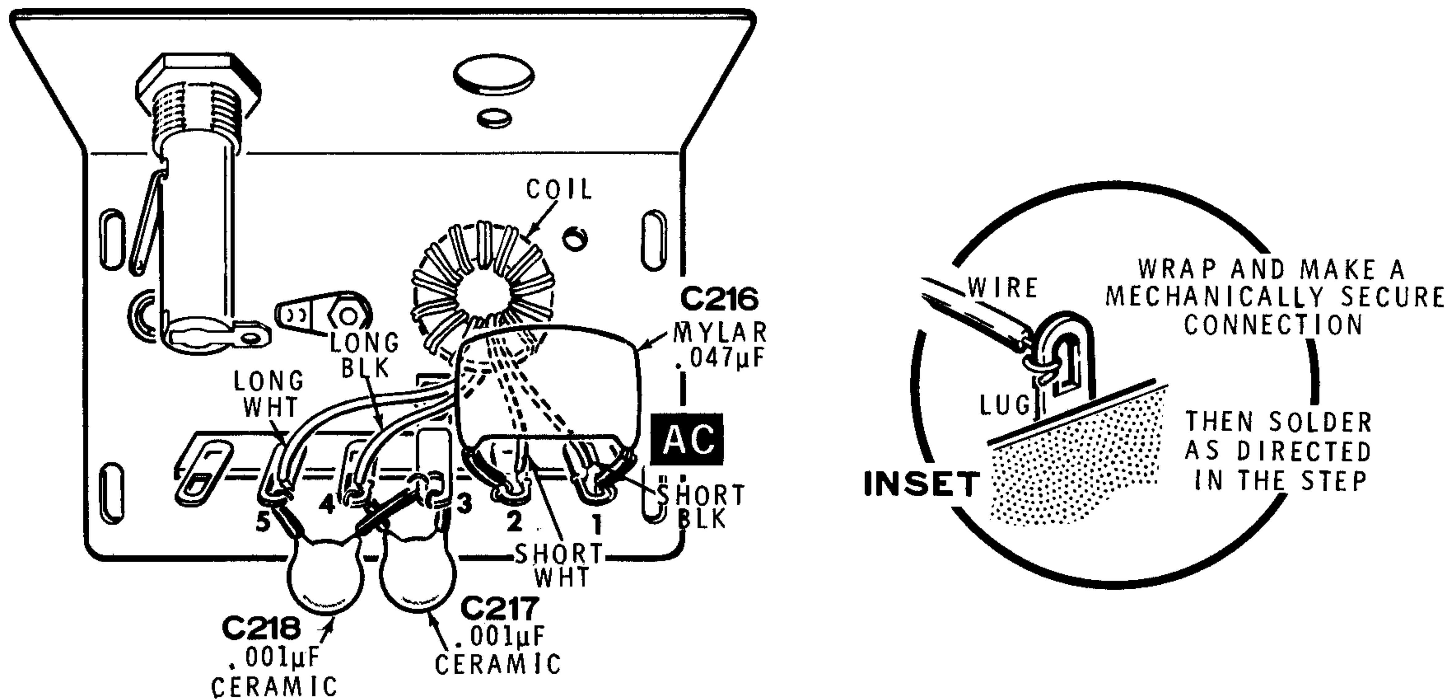
PICTORIAL 3-5
