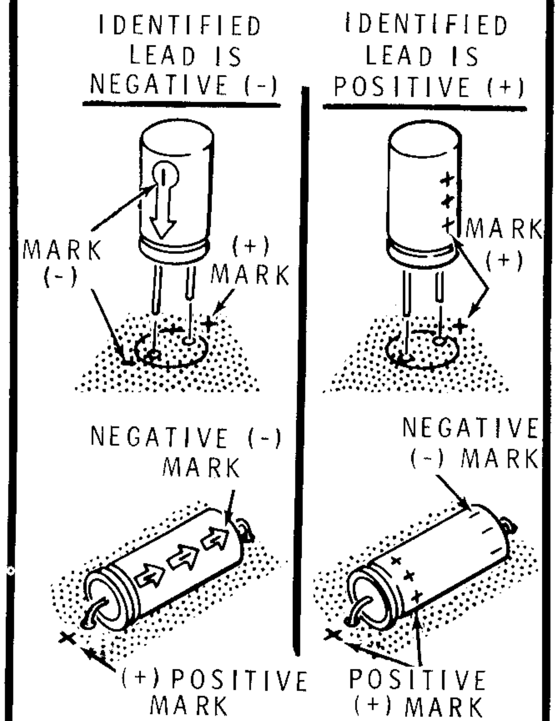
Detail 1-5A
