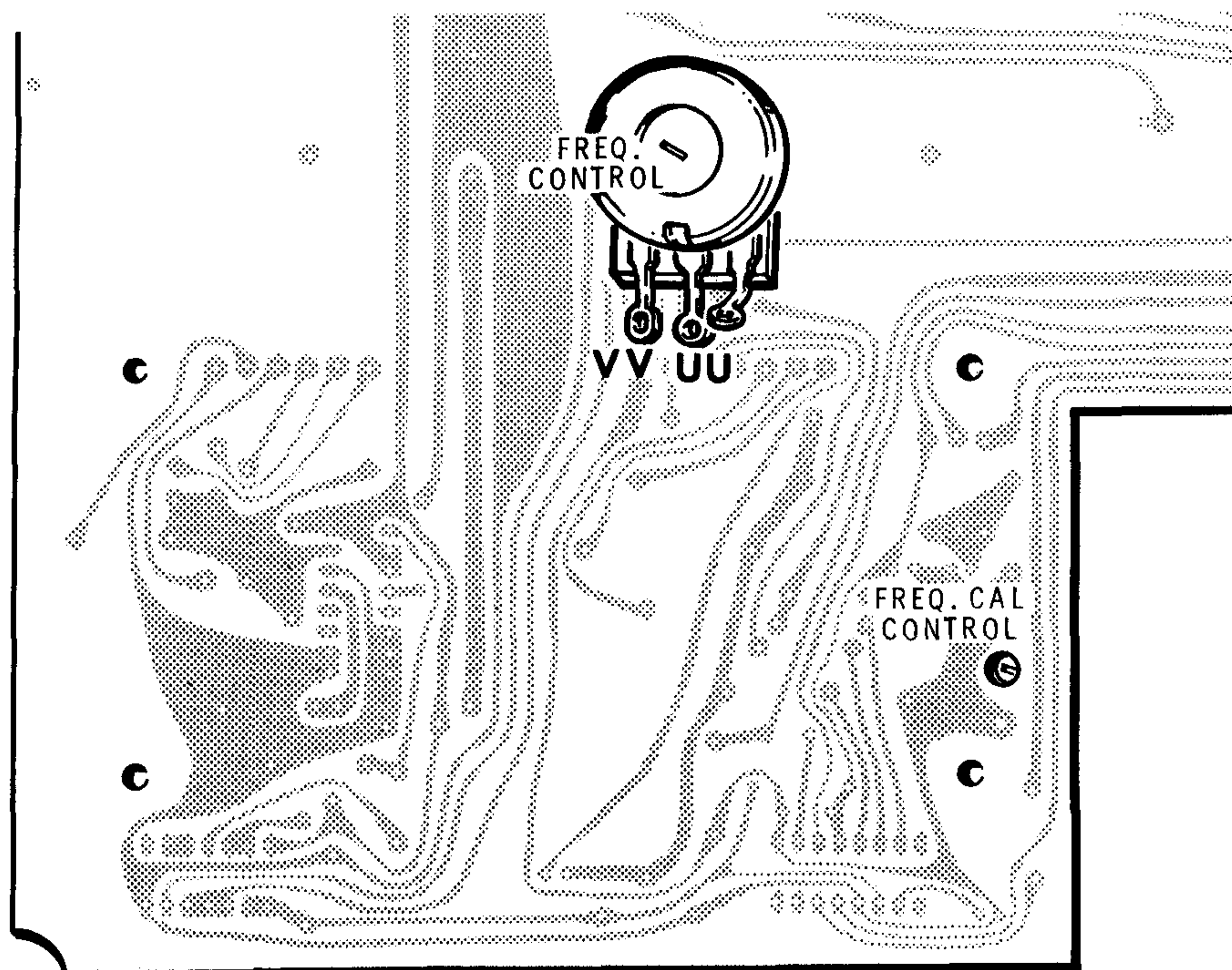
PICTORIAL 3-12
