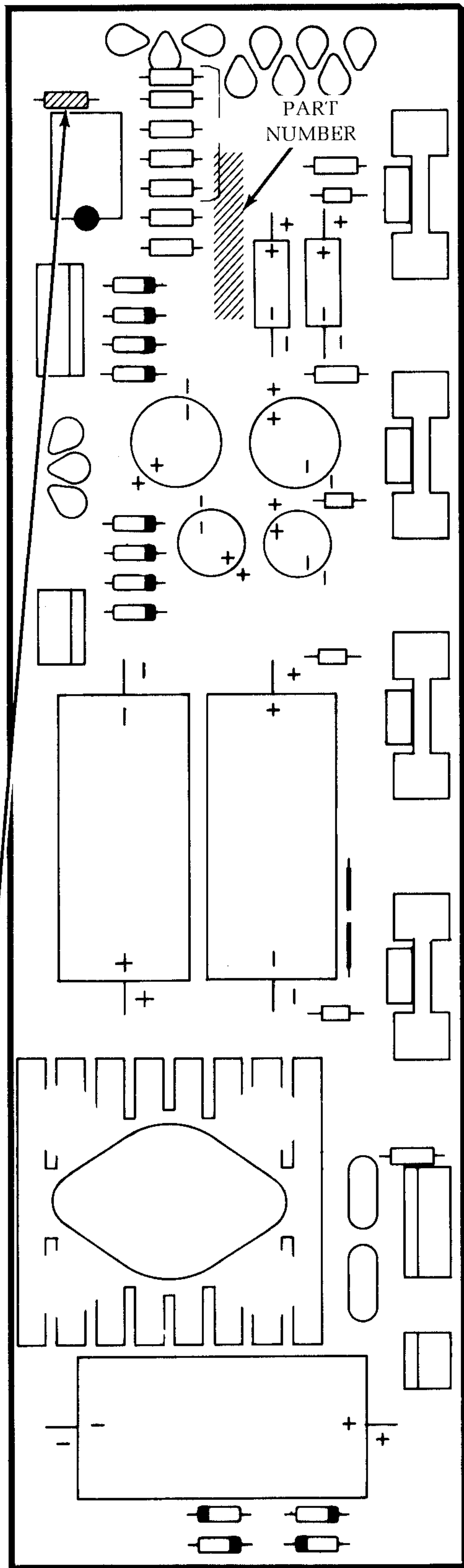
PICTORIAL 1-1
