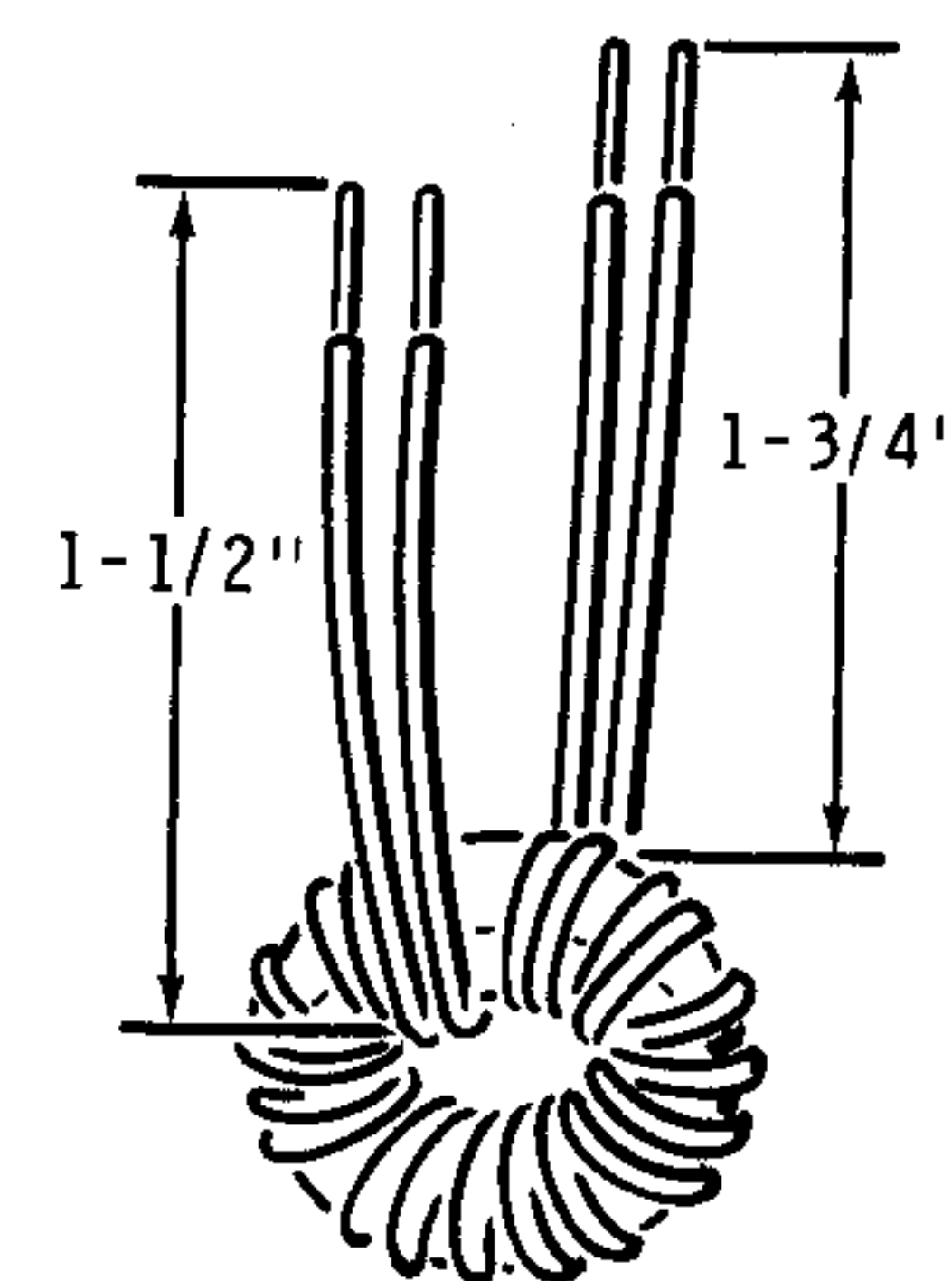
Detail 3-5A
