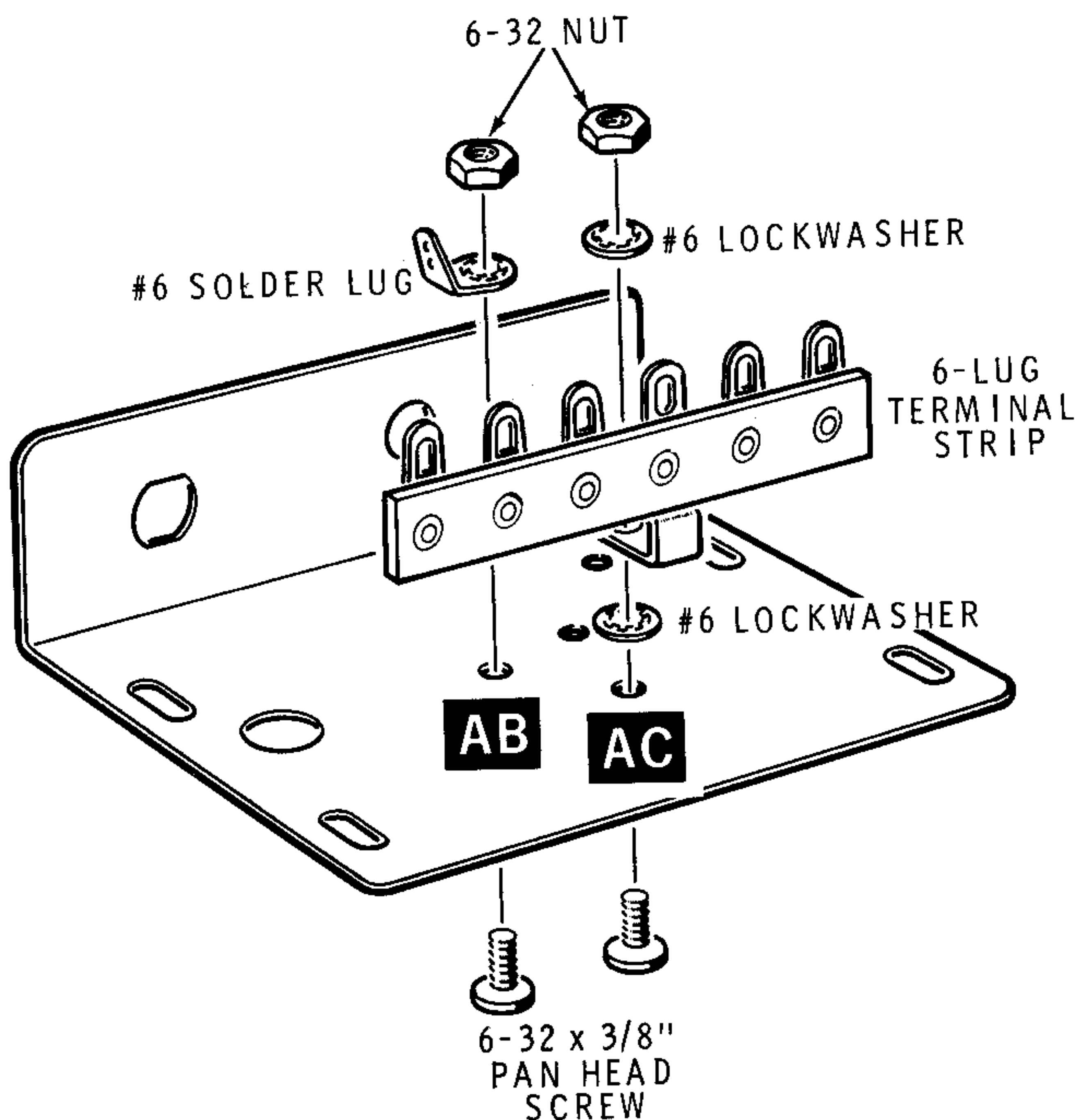
Detail 3-4A
