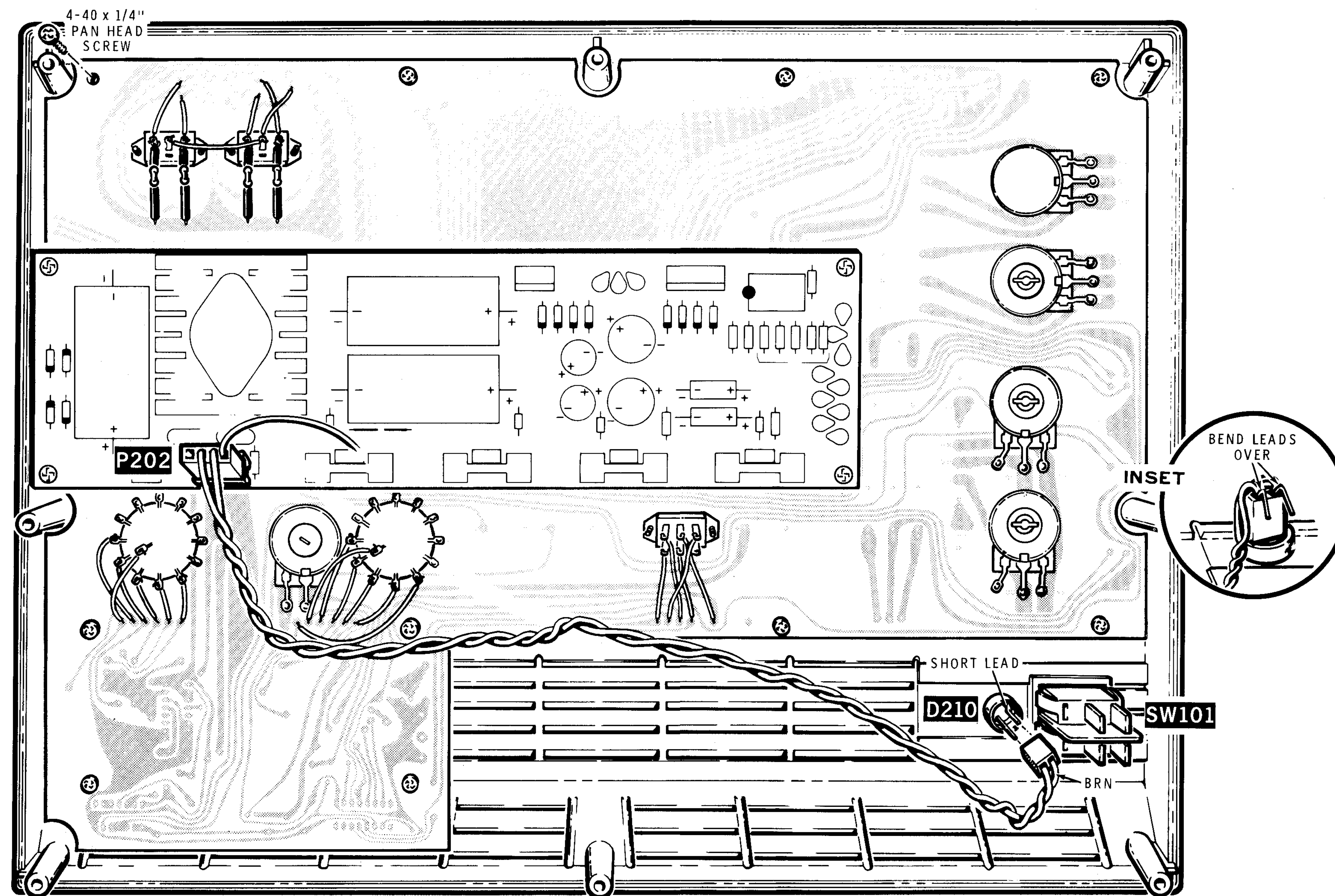
PICTORIAL 3-3
