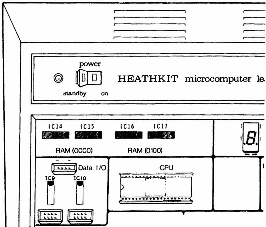
PICTORIAL 1-7
