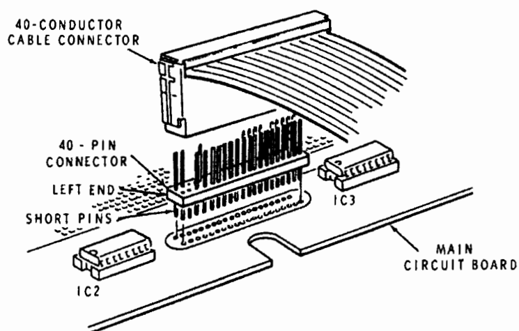
PICTORIAL 2-3
