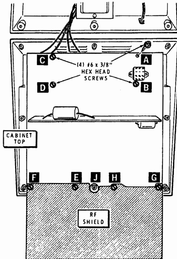
PICTORIAL 2-5
