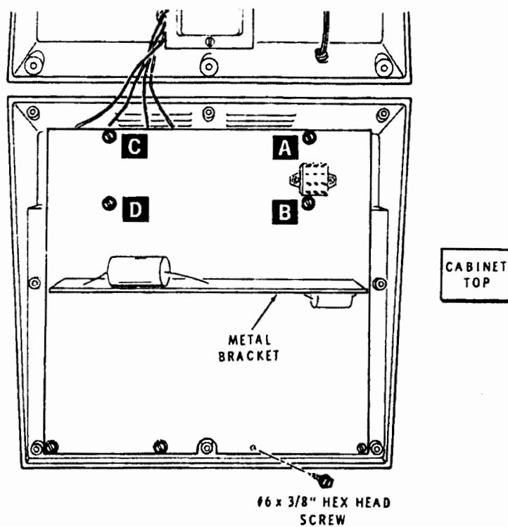
PICTORIAL 2-2
