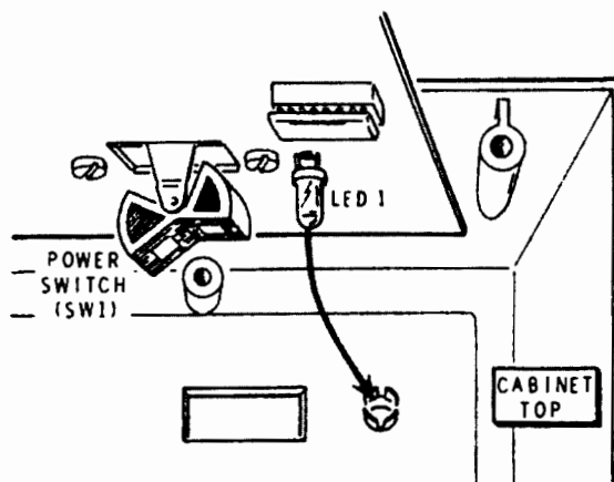
Detail 1-3A
