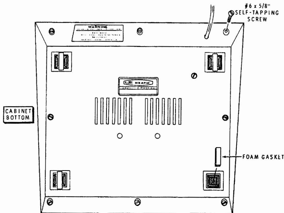
PICTORIAL 1-2
