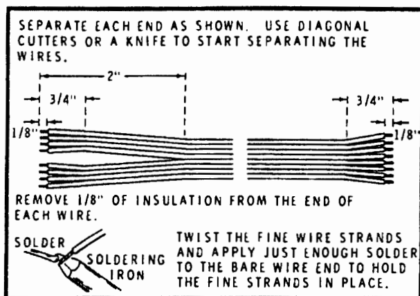
Detail 1-6A
