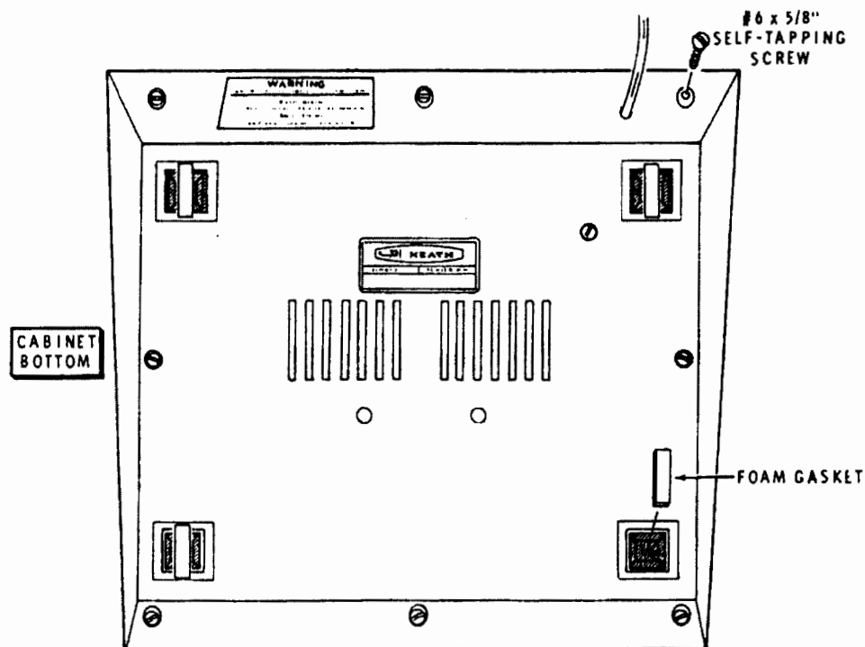
PICTORIAL 2-1
