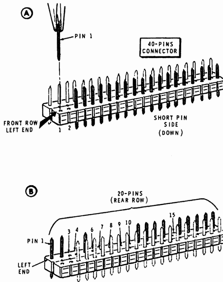
Detail 2-3A
