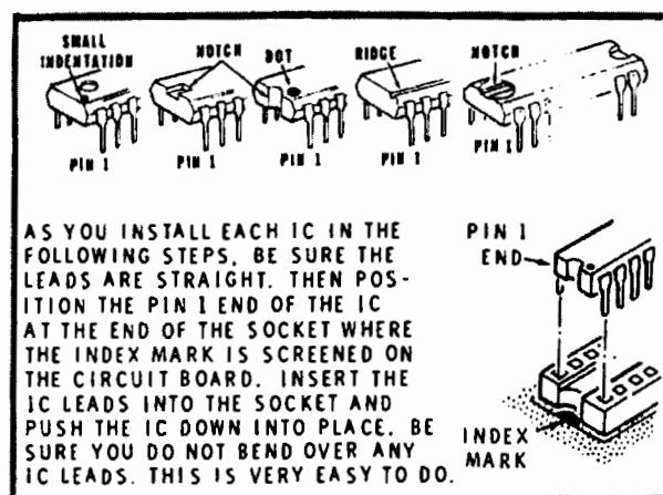
Detail 2-6B
