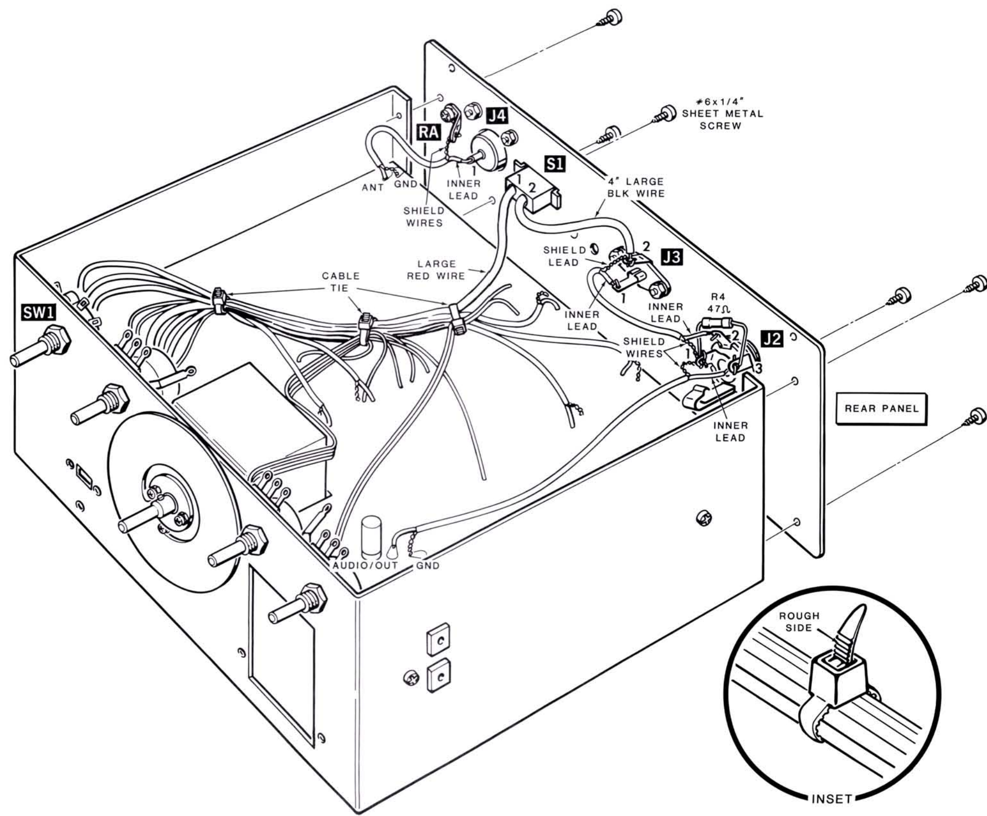
PICTORIAL 3-11
