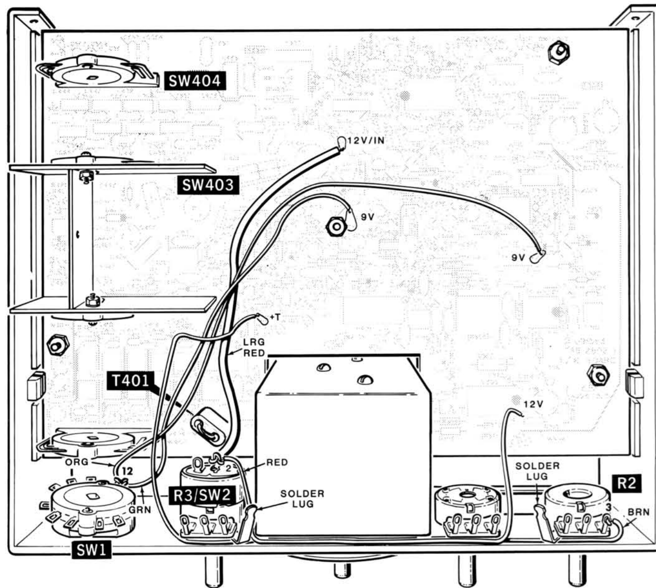
PICTORIAL 3-7
