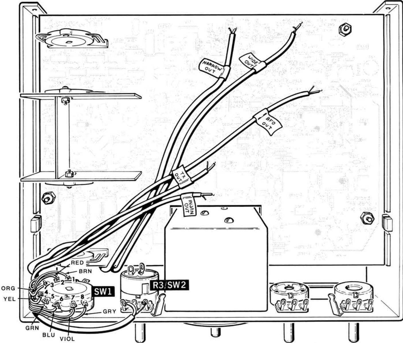
PICTORIAL 3-9
