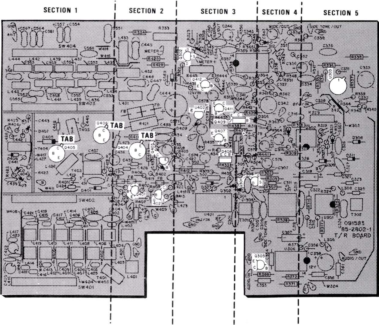
PICTORIAL 2-4
