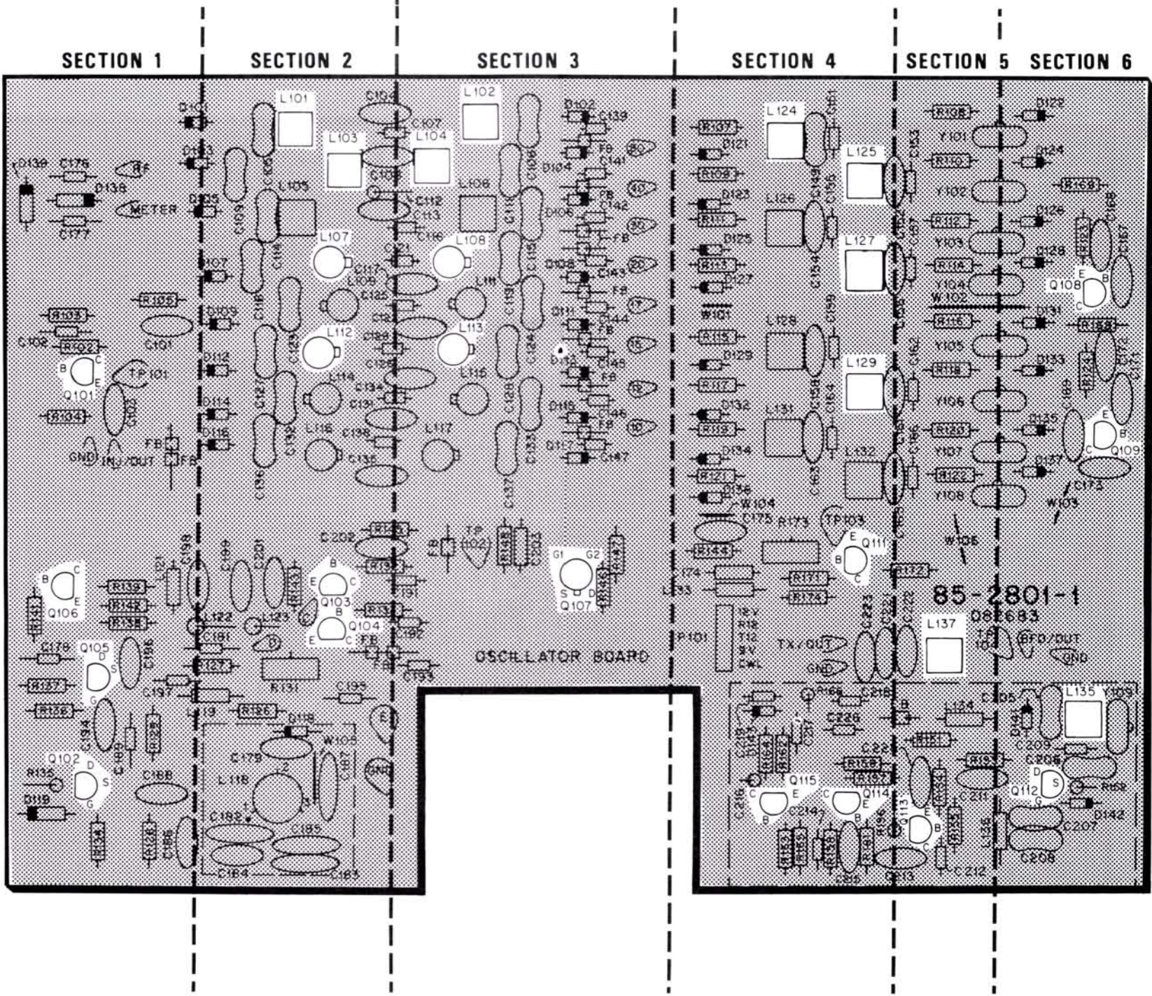
PICTORIAL 1-4
