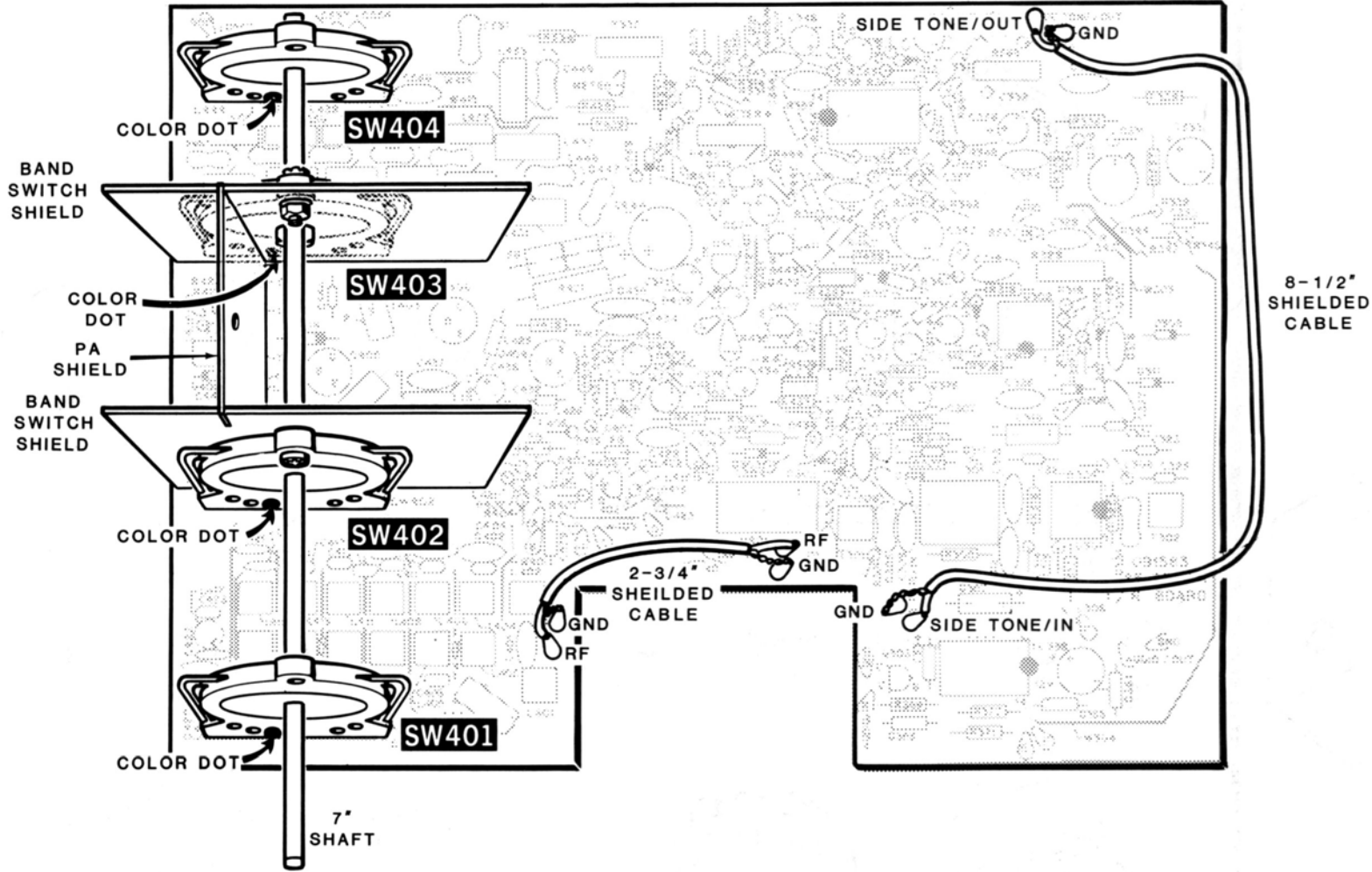
PICTORIAL 2-9
