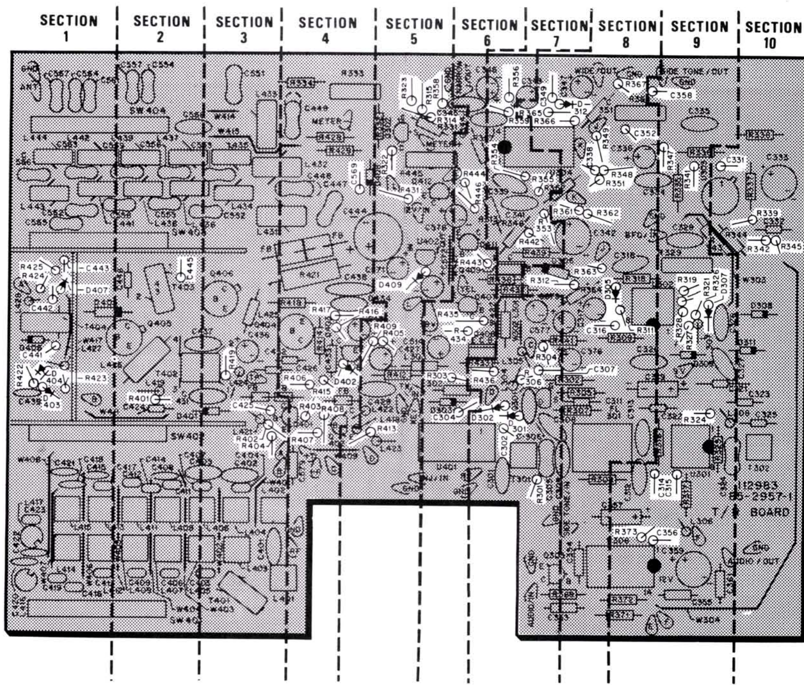
PICTORIAL 2-2
