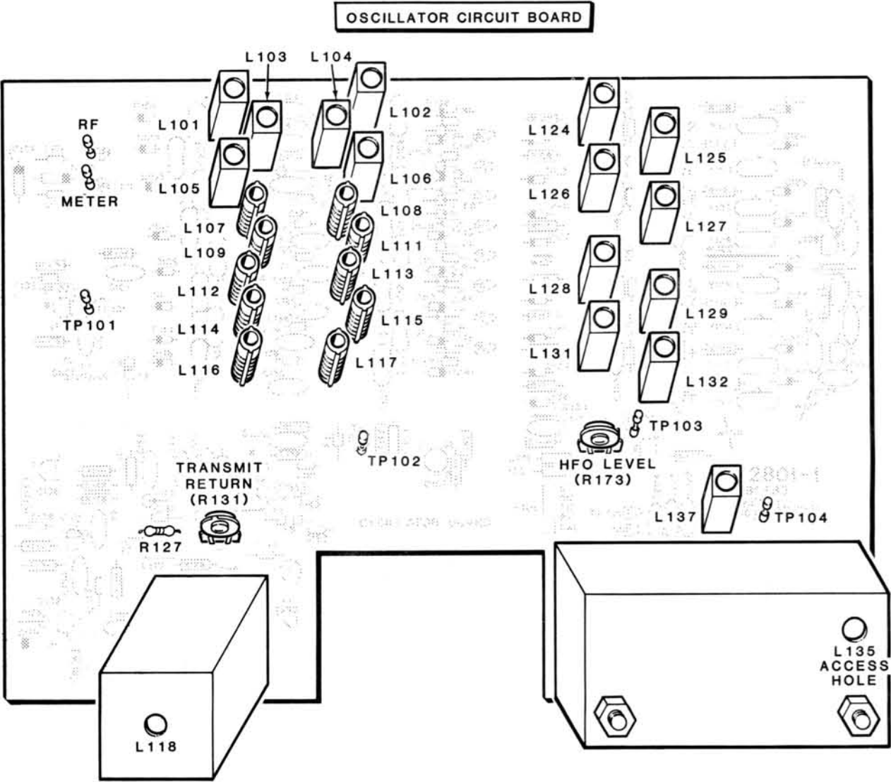
PICTORIAL 5-3
