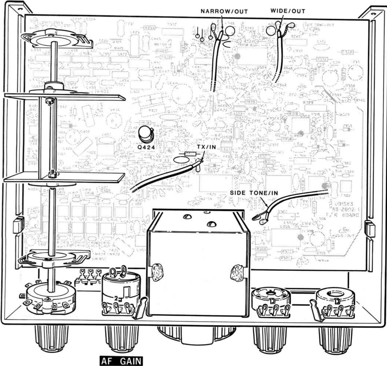
PICTORIAL 4-2
