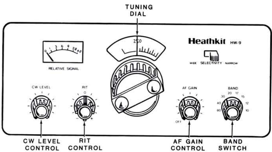
PICTORIAL 7-2
