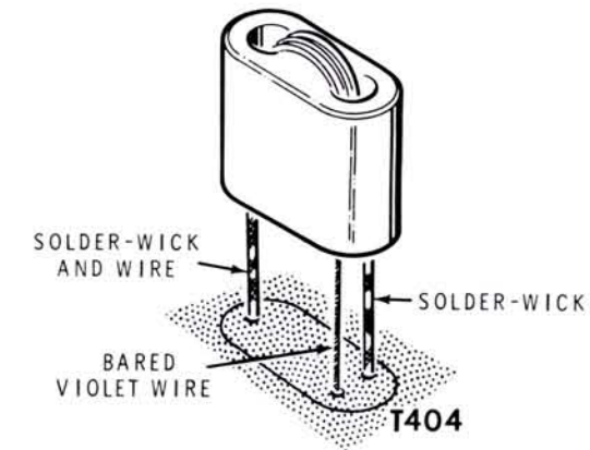
Detail 2-7B
