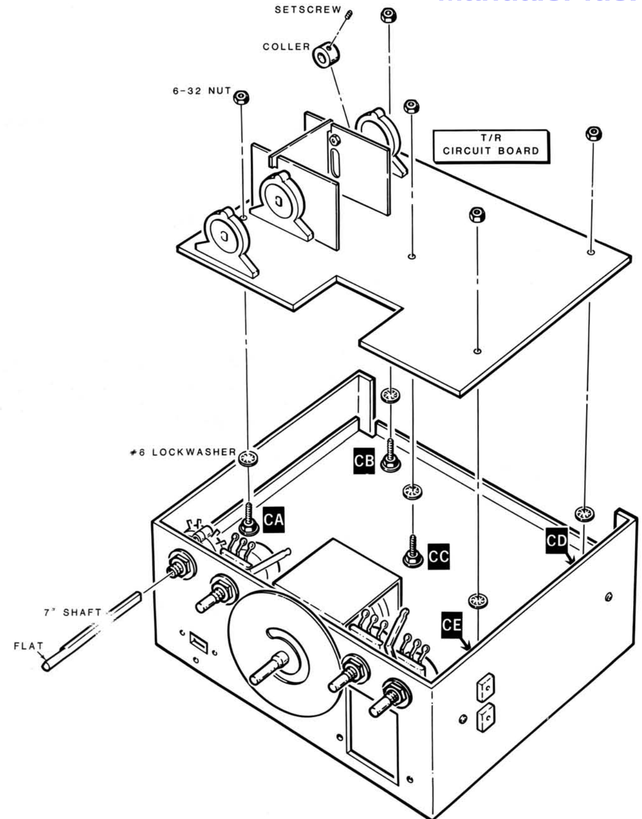
Detail 3-7A
