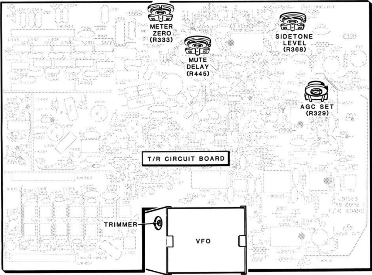
PICTORIAL 5-2
