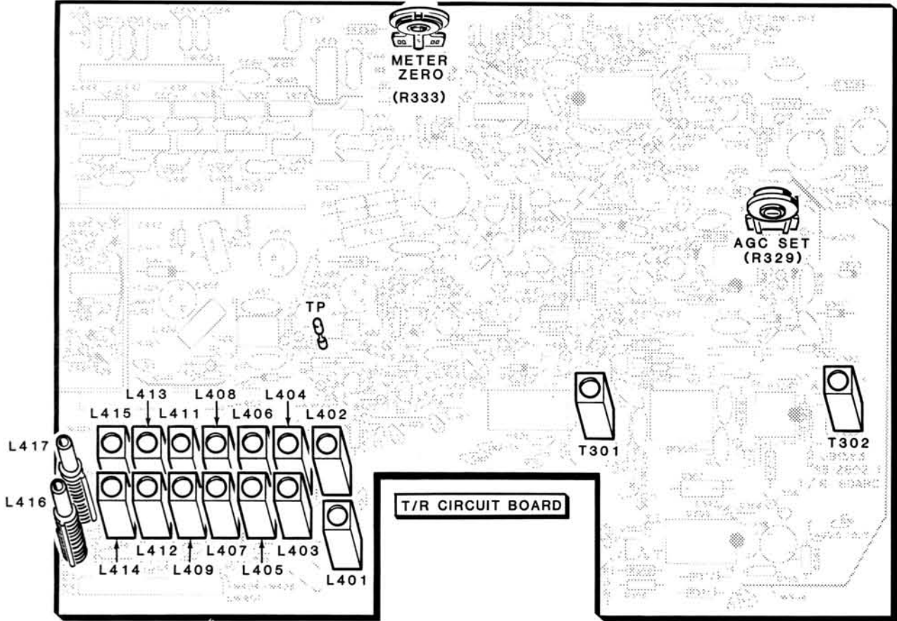
PICTORIAL 5-4
