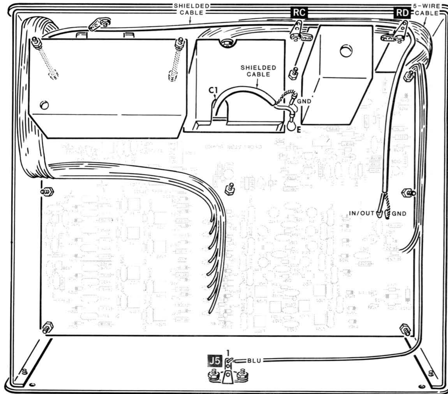
PICTORIAL 3-14
