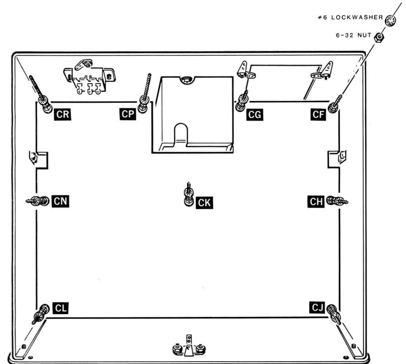
Detail 3-14A
