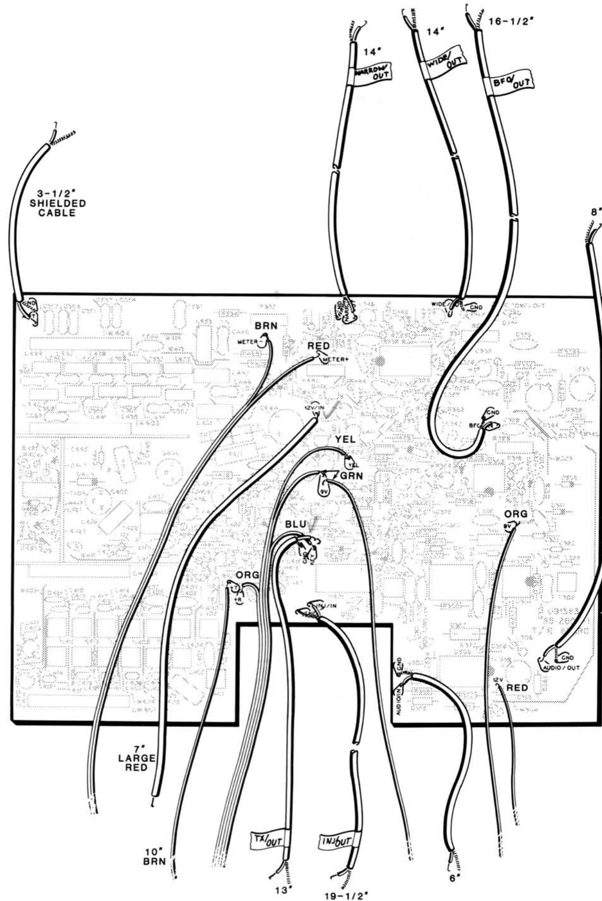
PICTORIAL 3-6
