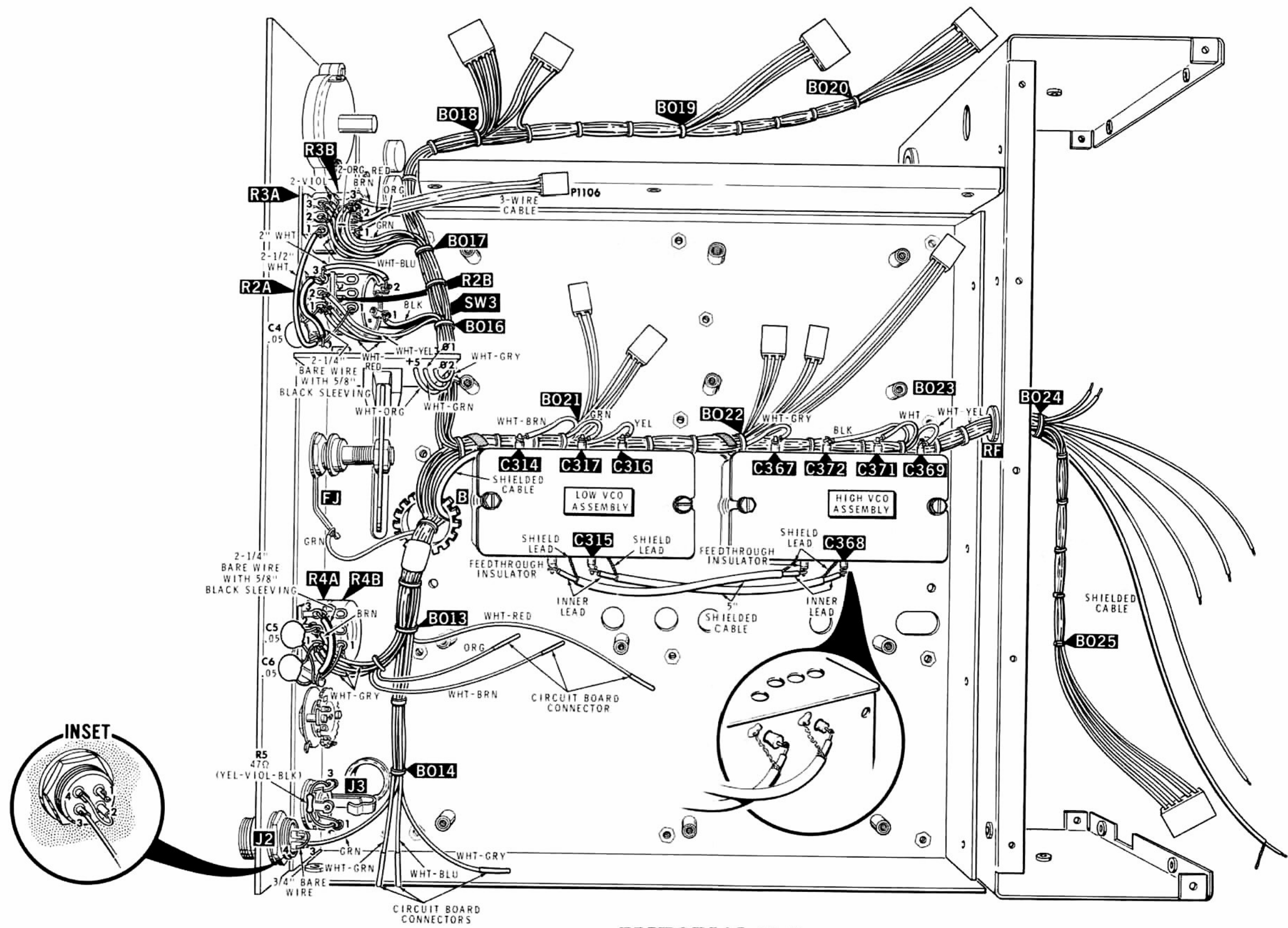
PICTORIAL 15-8
