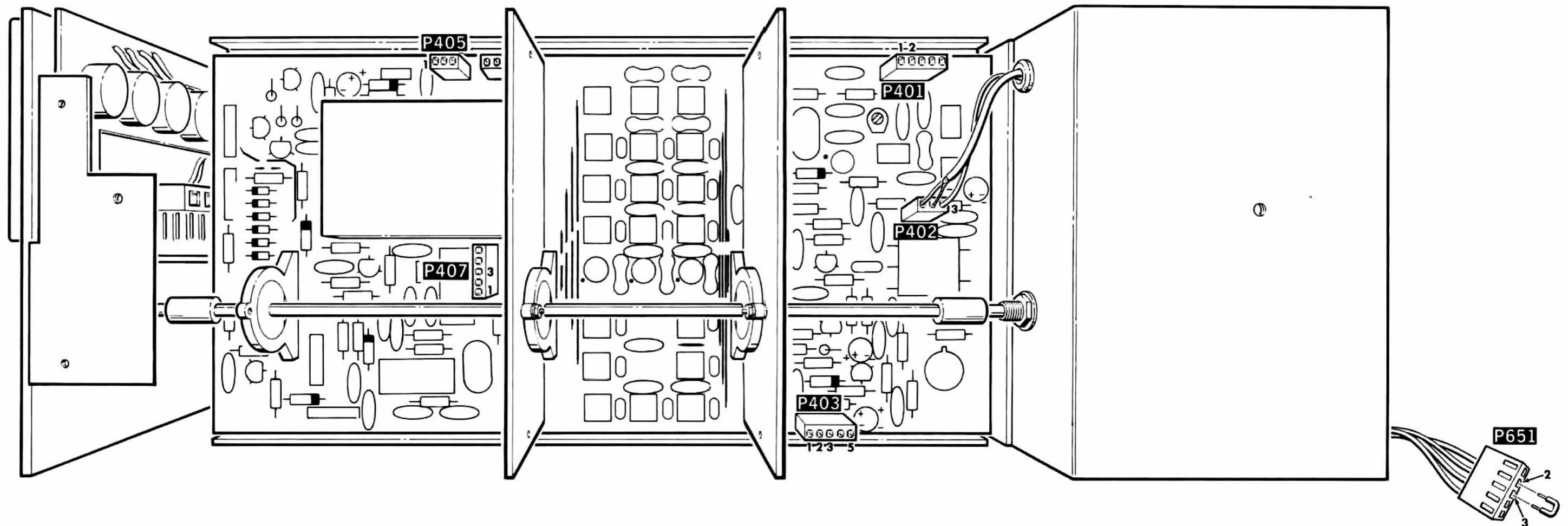
PICTORIAL 16-14
