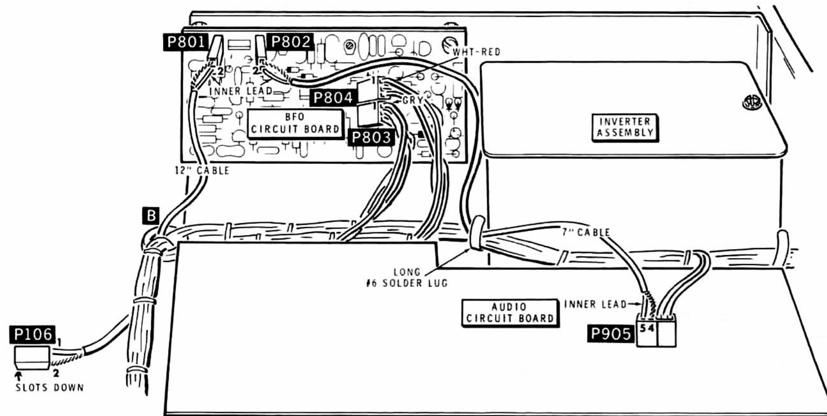
PICTORIAL 16-5
