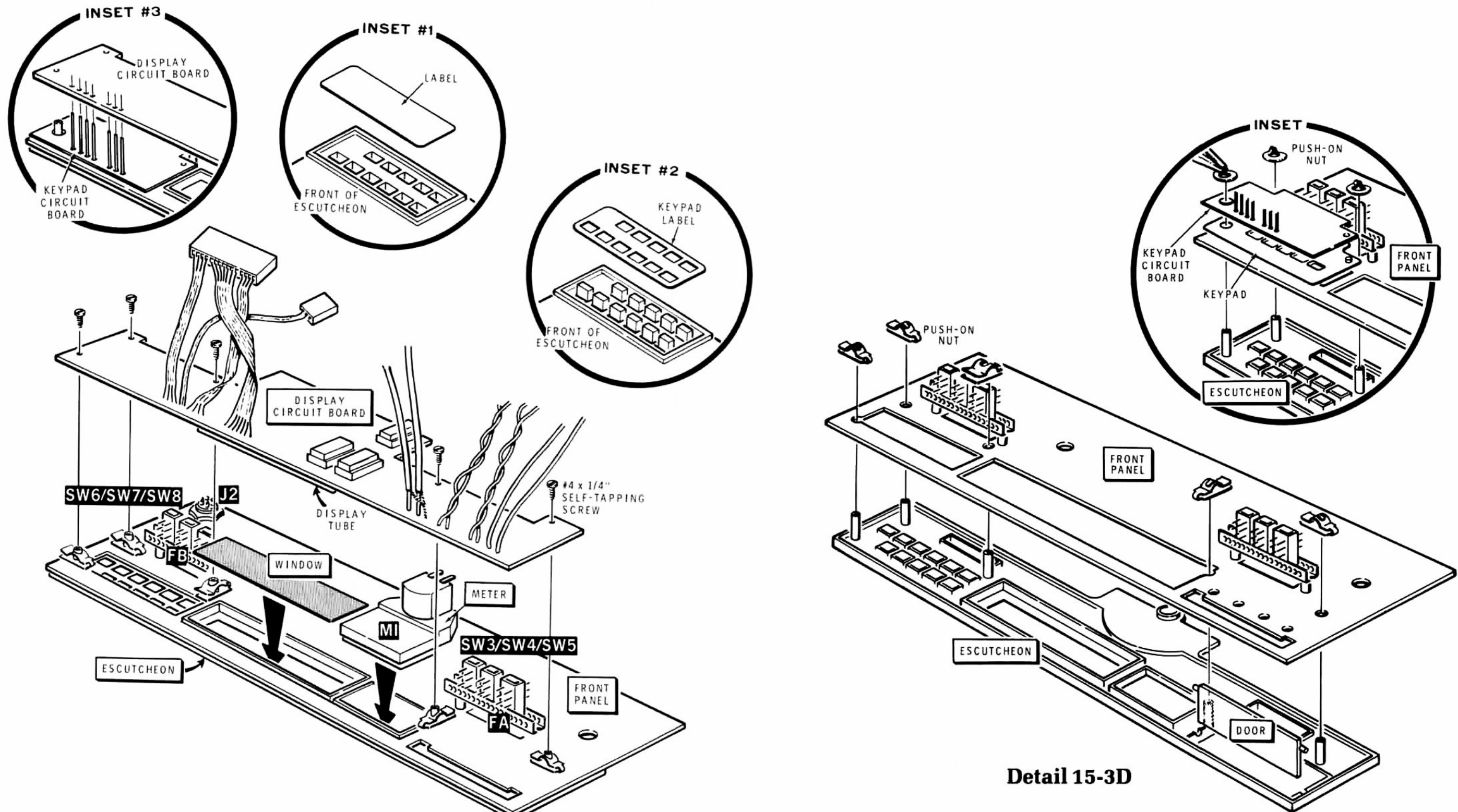
PICTORIAL 15-3
