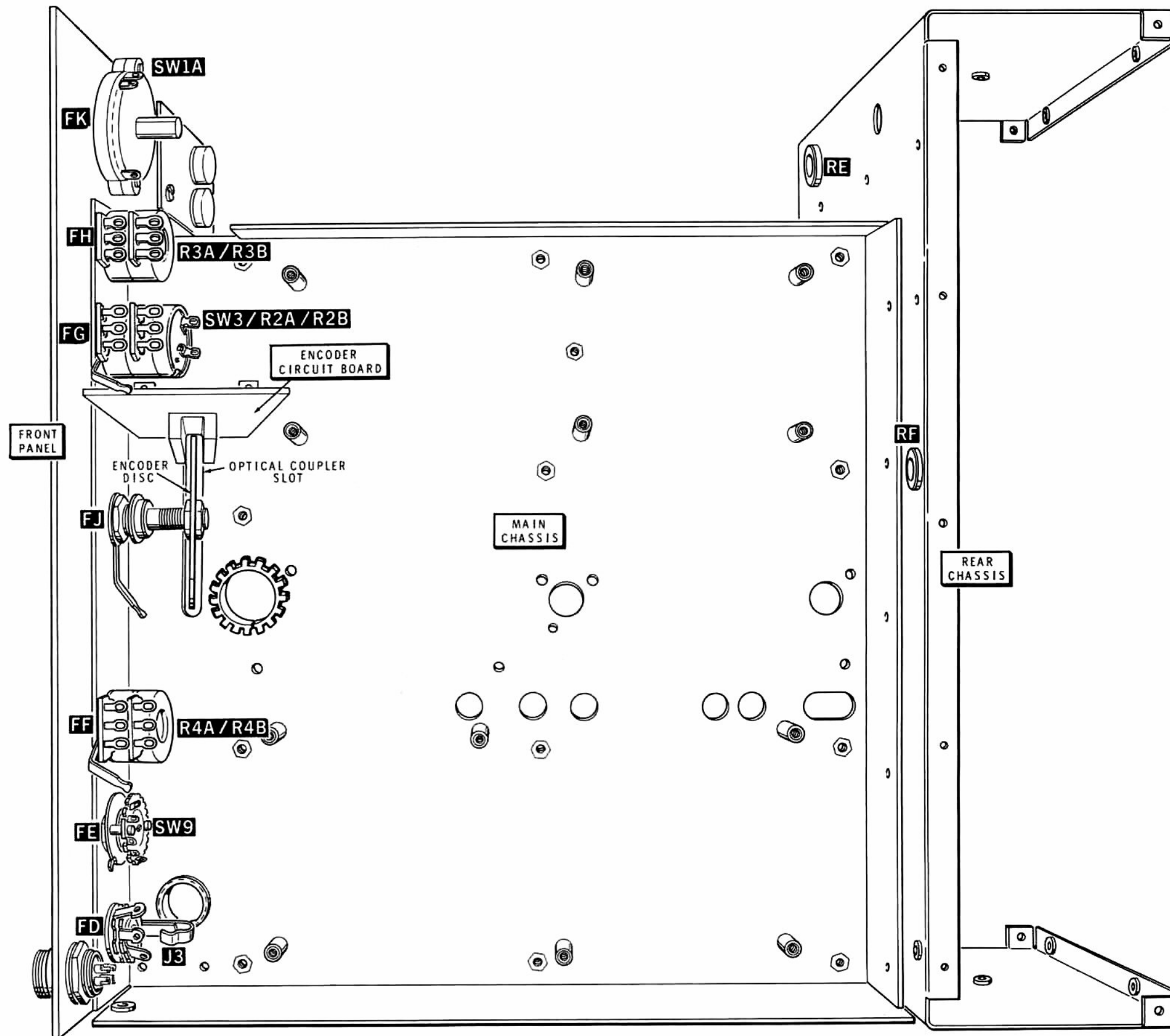
PICTORIAL 15-4
