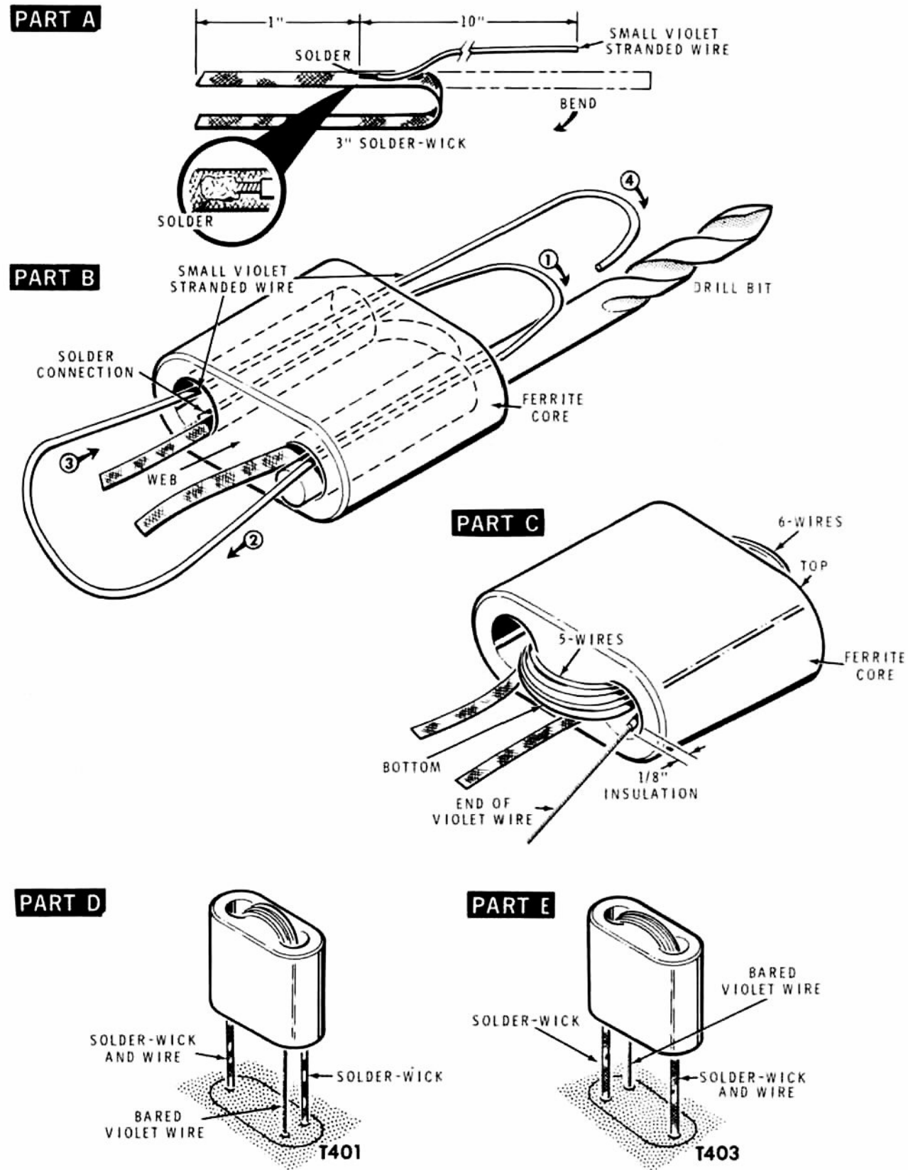
Detail 12-11B
