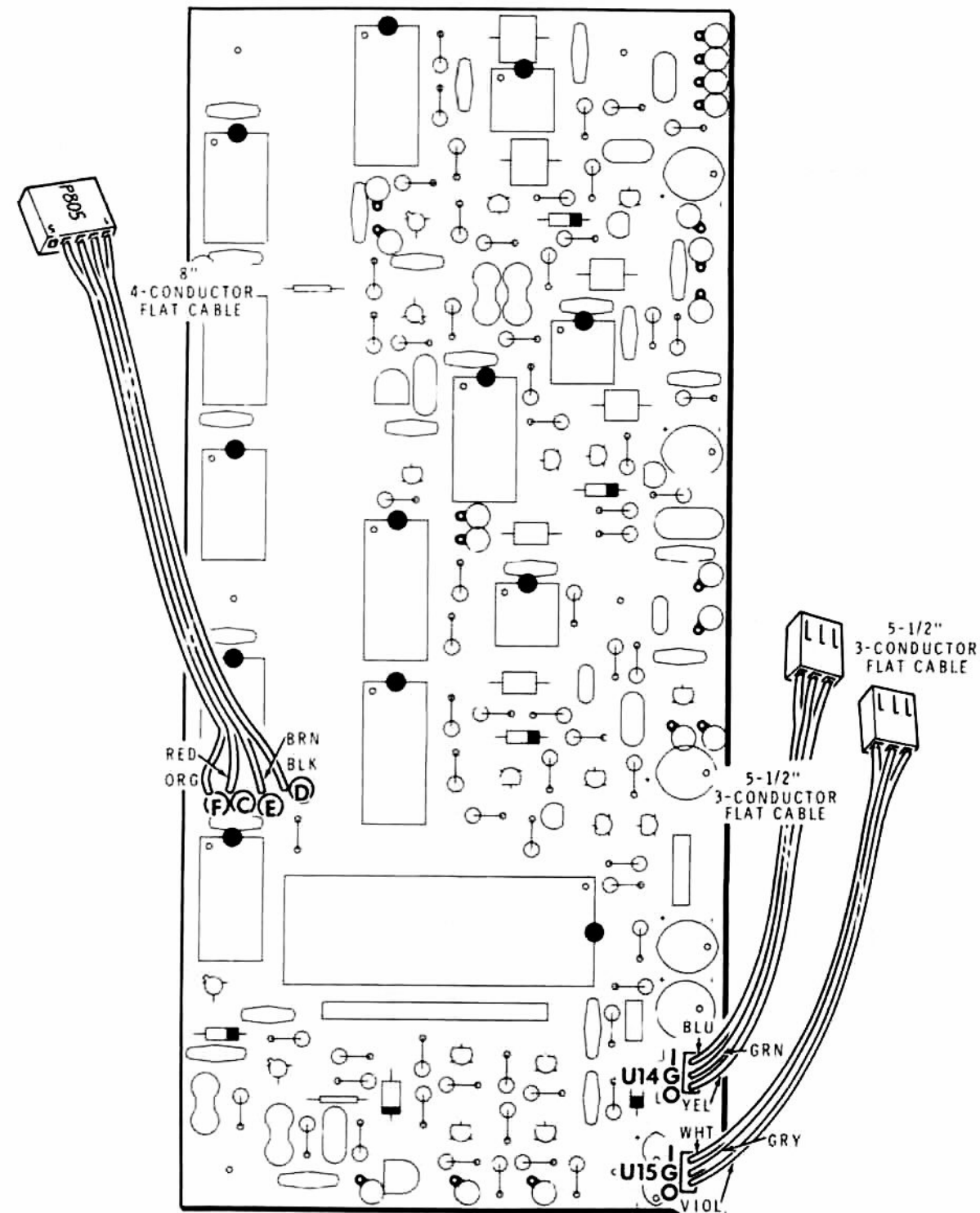
PICTORIAL 10-10
