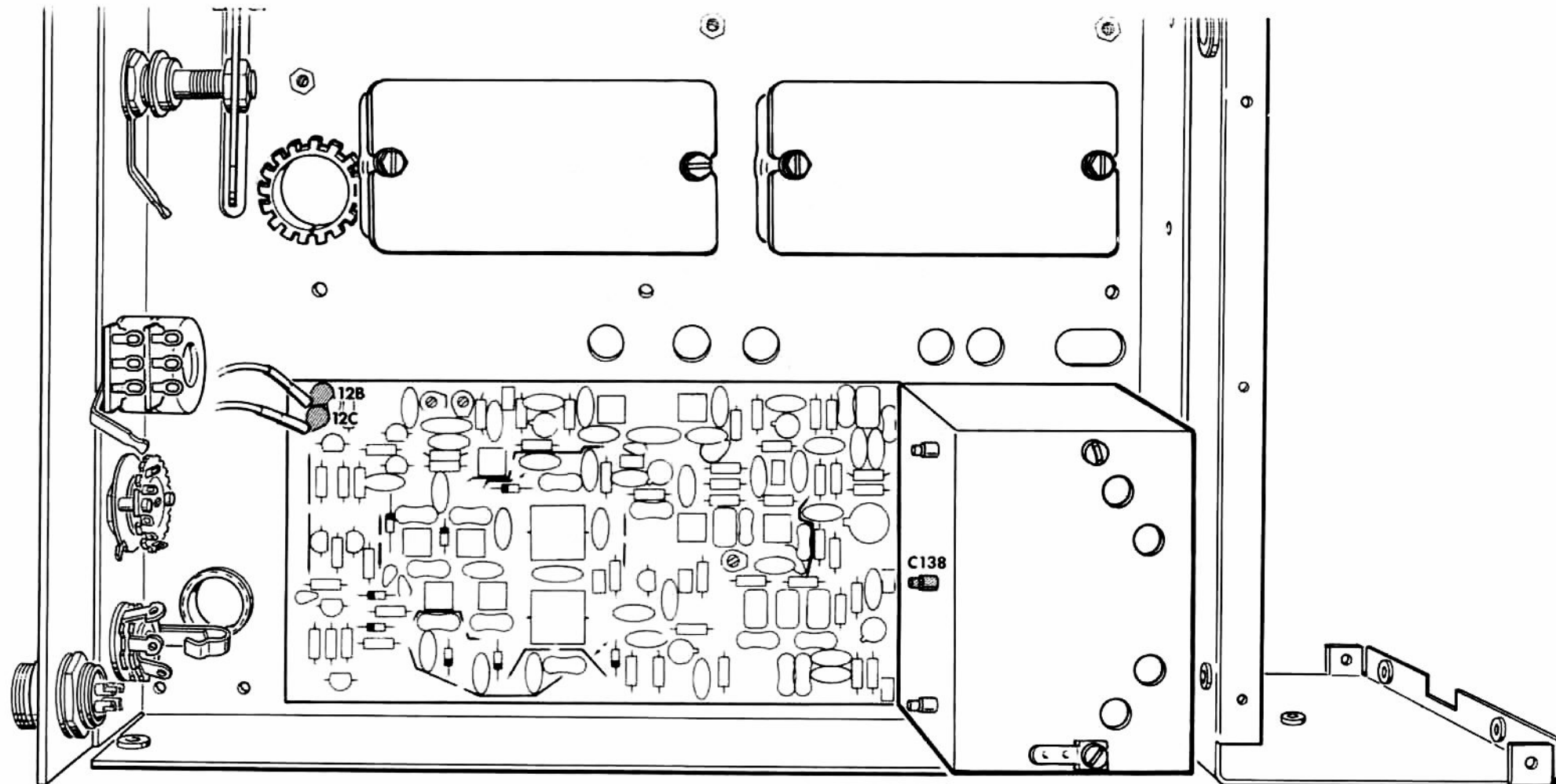
PICTORIAL 16-10
