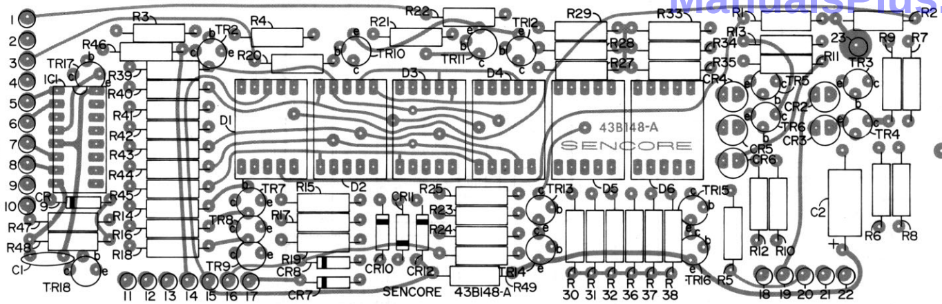
DISPLAY BOARD (COMPONENT SIDE)
