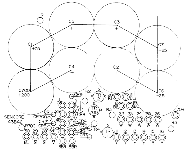
Fig. 5-B. Component side view.
