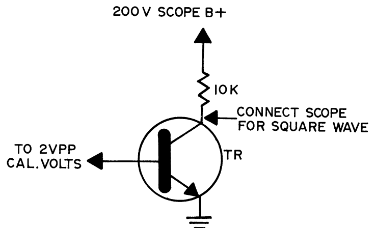
Circuit for 200V PP calibration square wave.
