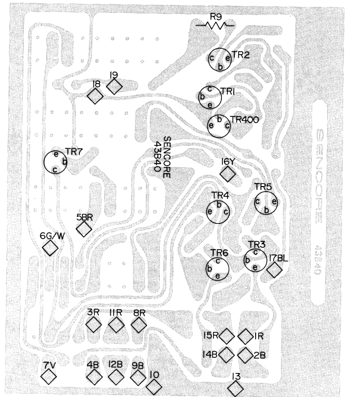
Fig. 4-B. Component side view.
