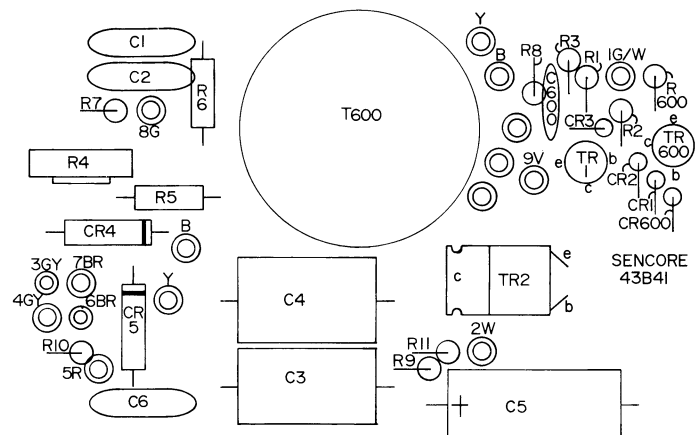
Fig. 6-B. Component side view.
