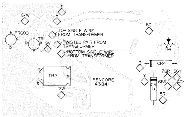
Fig. 6-A. Foil side view with board legend.
