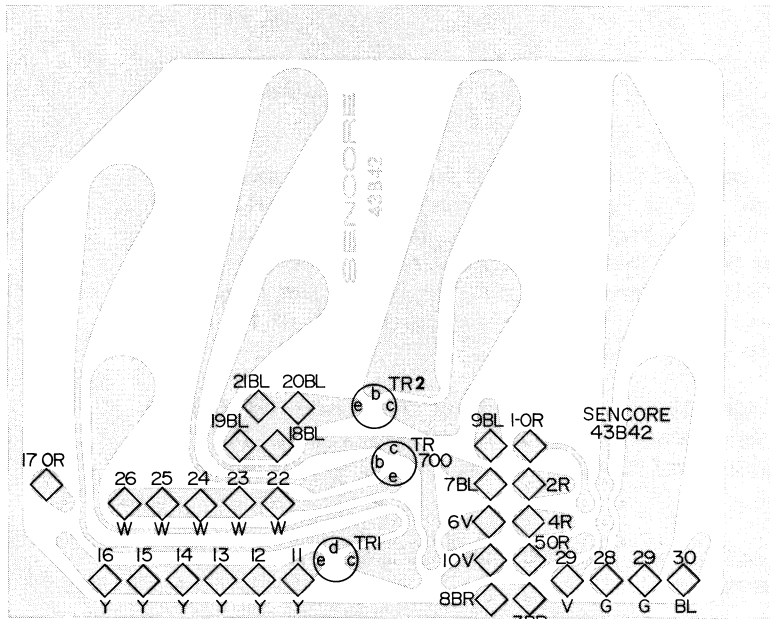
Fig. 5-A. Foil side view with board legend.
