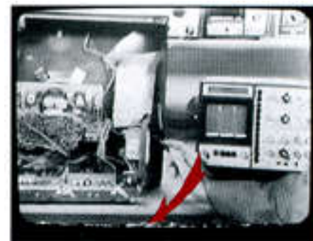
Fig. 2: Noise appears in the picture at the point where the VCR switches from one video head to the other. The switching adjustment keeps this noise close to the bottom of the screen, so that is not annoying.
