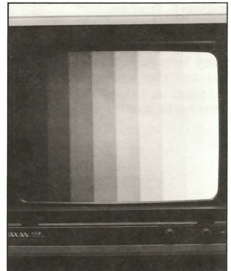
Fig. 7: The 10-Bar Staircase pattern tests the video stages for correct dynamic operating range, from pure black to pure white.
