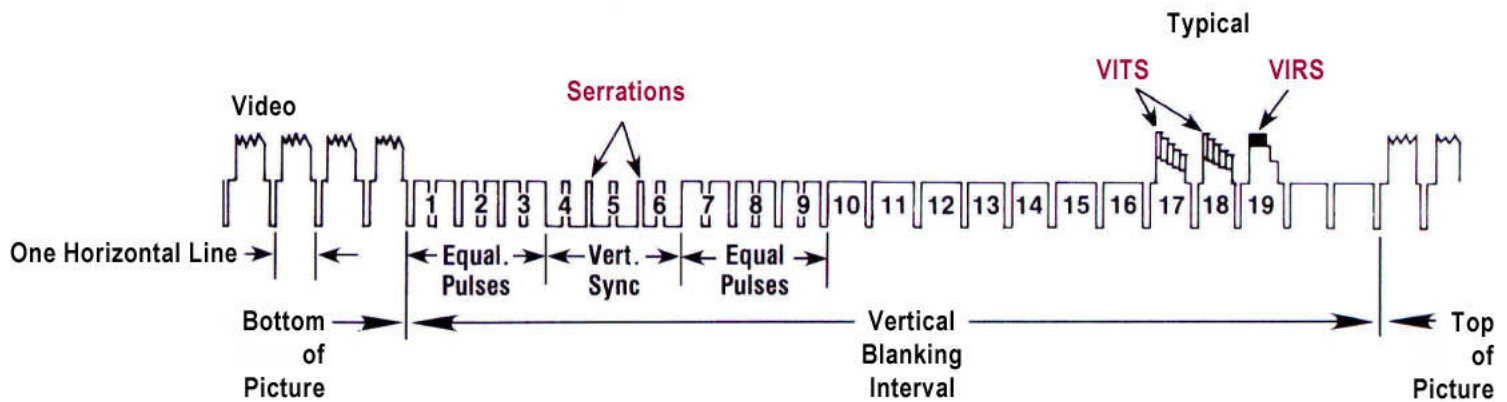
Fig. 4: Detail of the vertical blanking interval.
