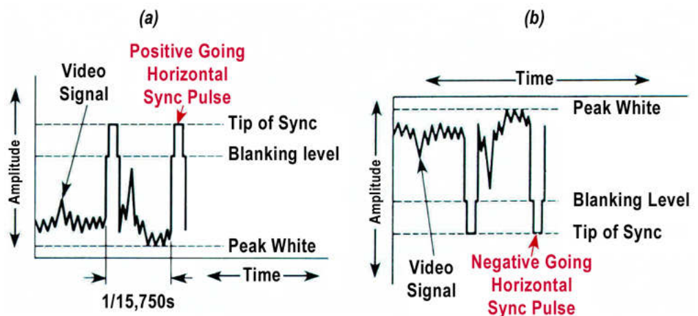
Fig. 1: (a) Two horizontal lines of composite video with positive sync. (b) Same video signal as (a), but with negative sync polarity.
