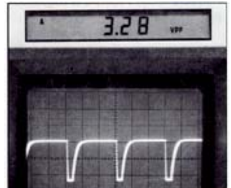
Fig. 3: Use the Waveform Analyzer's DIGITAL READOUT functions and the CRT to isolate defective sensors.
