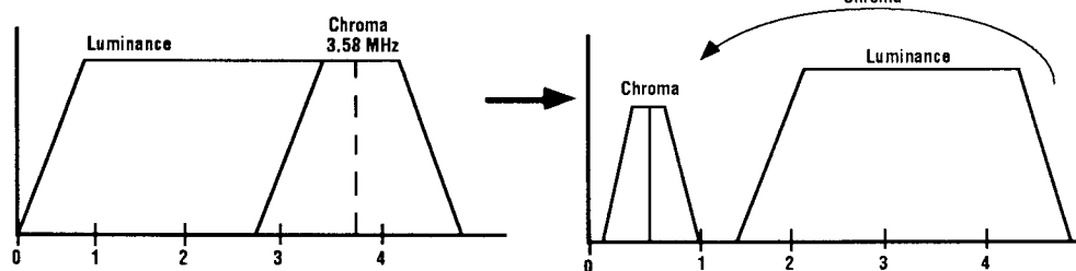
Fig 1: The frequency of the chroma signal is down-converted in the VCR "color under" format.
