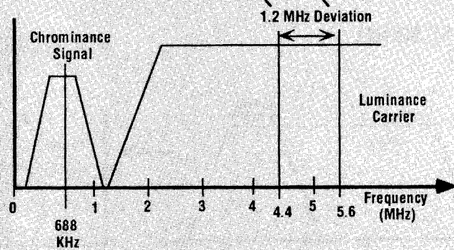
Fig. 4: The Super Beta format raises the luminance frequency to improve resolution from the existing format.
