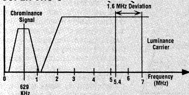
Fig. 3: VHS Super formats raise the luminance frequency to improve resolution from the existing format.
