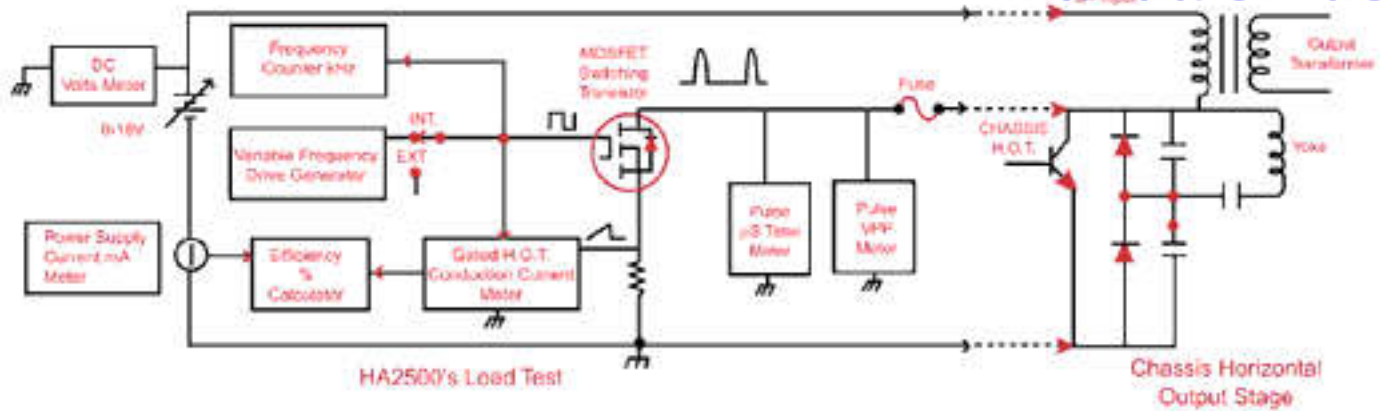
Fig. 2: Block diagram of the Load Test and connections to a horizontal output stage.
