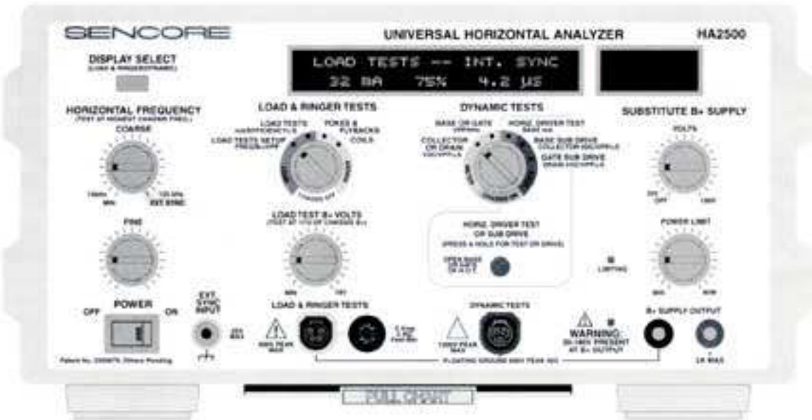
Fig. 1: The Load Tests of the Sencore HA2500 Universal Horizontal Analyzer test horizontal output stages with no AC power applied to the chassis.
