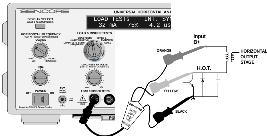
Fig. 1: The three LOAD TESTS readouts determine if the horizontal output stage is normal or contains a defect.
