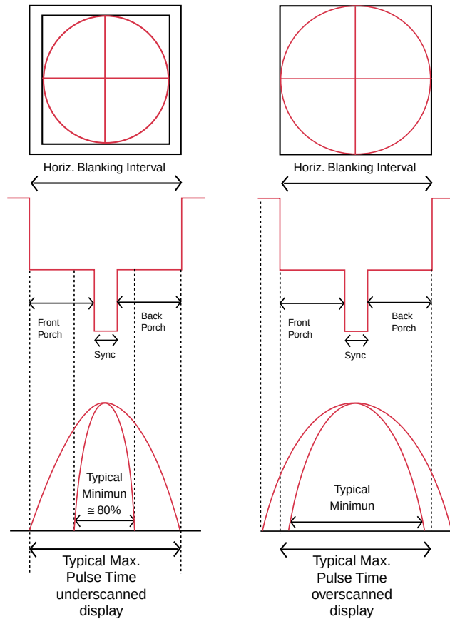
Fig. 2: Typical pulse \mu S times relate to the horizontal blanking interval and overscan or underscanned characteristics of the display.
