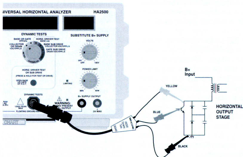
Fig. 2: The COLLECTOR OR DRAIN and BASE OR GATE Dynamic Tests require three simple DYNAMIC TEST LEAD connections to the horizontal output transistor.
