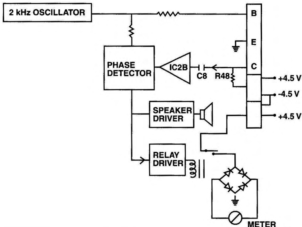
Fig. 18: Block Diagram for Cricket Gain Test.
