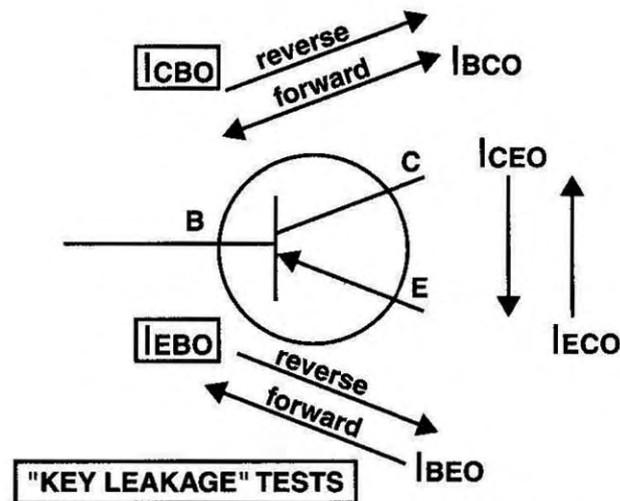
Fig. 11: Leakage Paths for a PNP Transistor.
