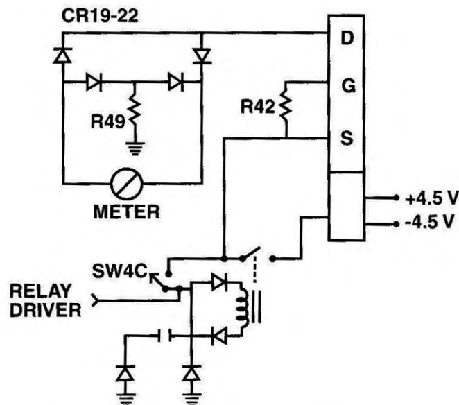
Fig. 23: Idss Leakage Test Circuit.
