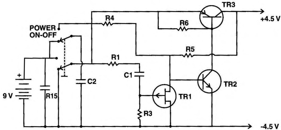
Fig. 24: Auto-Off Circuit
