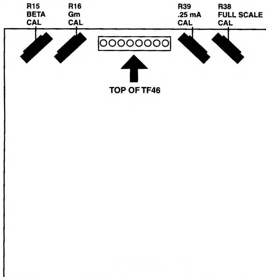
Fig. 28: Location of Calibration Controls on P.C. Board.
