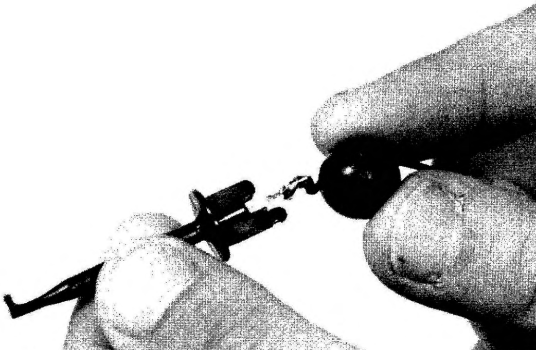
Fig. 26: Disassembly of E-Z Hook® for service.
