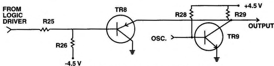
Fig. 19: Details of Phase Detector Circuit.
