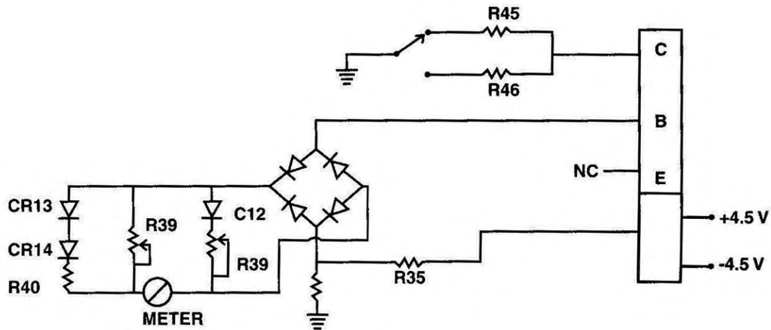
Fig. 22: Leakage Test Circuit.
