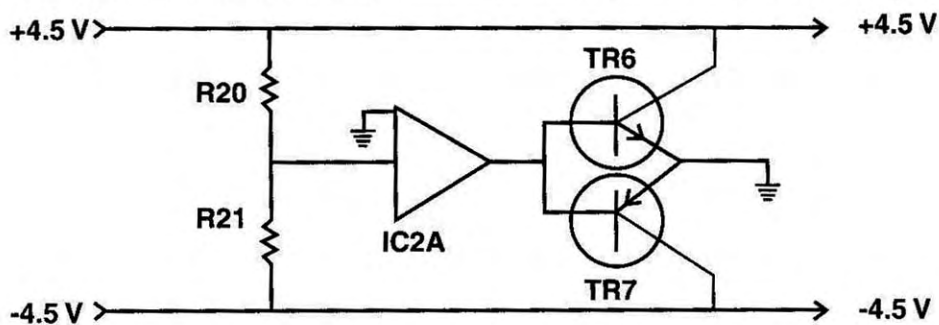
Fig. 25: Supply Splitter Circuit
