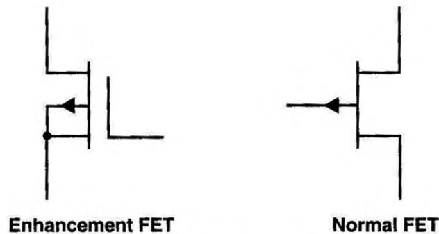
Fig. 16: Schematic Symbol for Enhancement FET.
