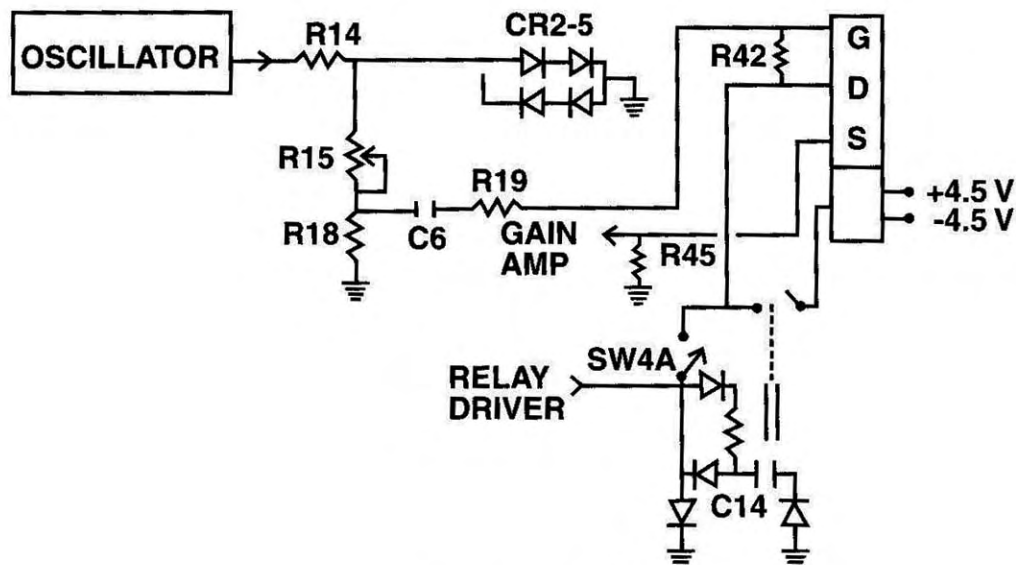
Fig. 21: FET Gm Gain Test.
