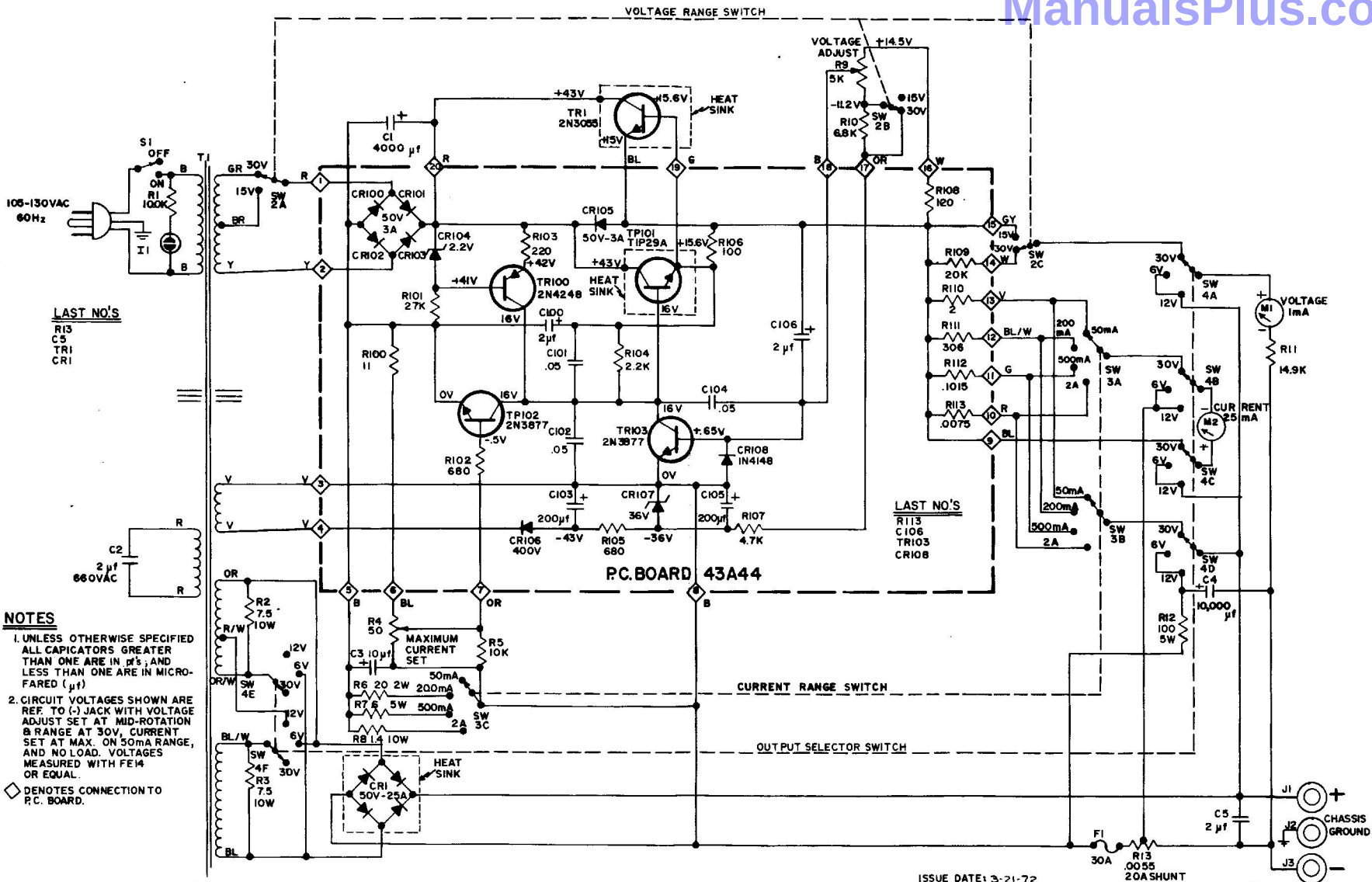
SCHEMATIC DIAGRAM UPS I64
